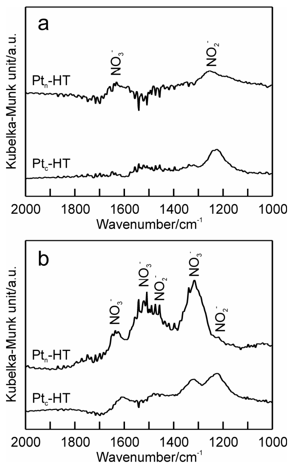
Figure 1. In situ DRIFT spectra of NO x adsorbates on Pt c -HT and Pt n -HT after exposing to streams of a) 0.08%NO, He balance. b) 0.08%NO, 10%O 2 , He balance.
