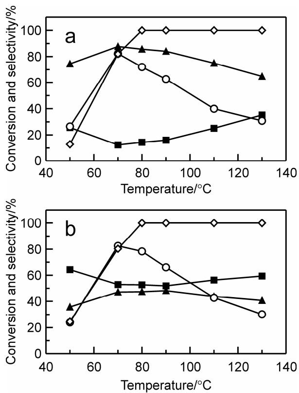
Figure 4. Conversion and selectivity of a) Pt c -HT and b) Pt n -HT. (○) NO x conversion, (◇) H 2 conversion, (■) N 2 selectivity, (▲) N 2 O selectivity. 0.08% NO, 10% O 2 , 0.28% H 2 , balanced with He, W/F=0.24 s·g·cm -3 .
