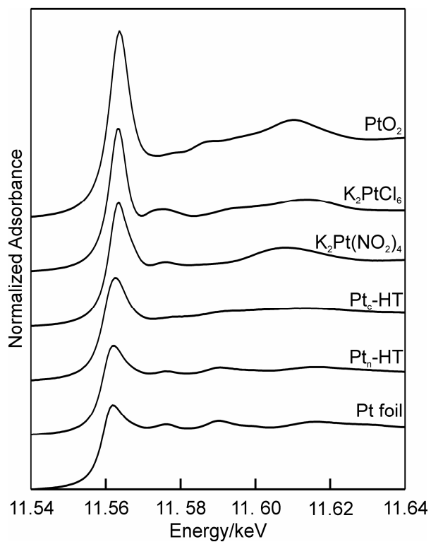
Figure 2. Normalized Pt L_{III} -XANES spectra.
