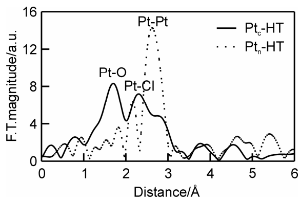
Figure 3. Pt L_{III} edge Fourier transform EXAFS of Pt_c -HT and Pt_n -HT after heating at 600 °C in H_2 .
