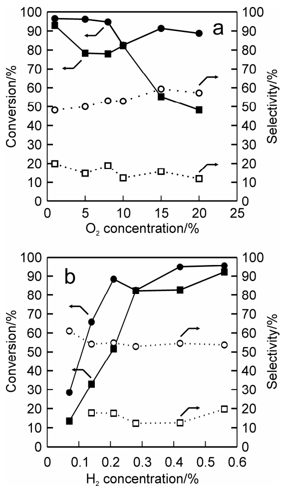
Figure 5. Effects of (a) O 2 concentration and (b) H 2 concentration on NO x conversion and N 2 selectivity at 70 °C. Pt c -HT; (■) NO x conversion and (□) N 2 selectivity. Pt n -HT; (●) NO x conversion and (○) N 2 selectivity. 0.08% NO, 1-20% O 2 , 0.07-0.56% H 2 , balanced with He, W/F=0.24 s·g·cm -3 .
