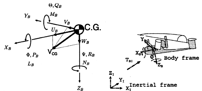
Fig. 3. Body frame and inertial frame.
