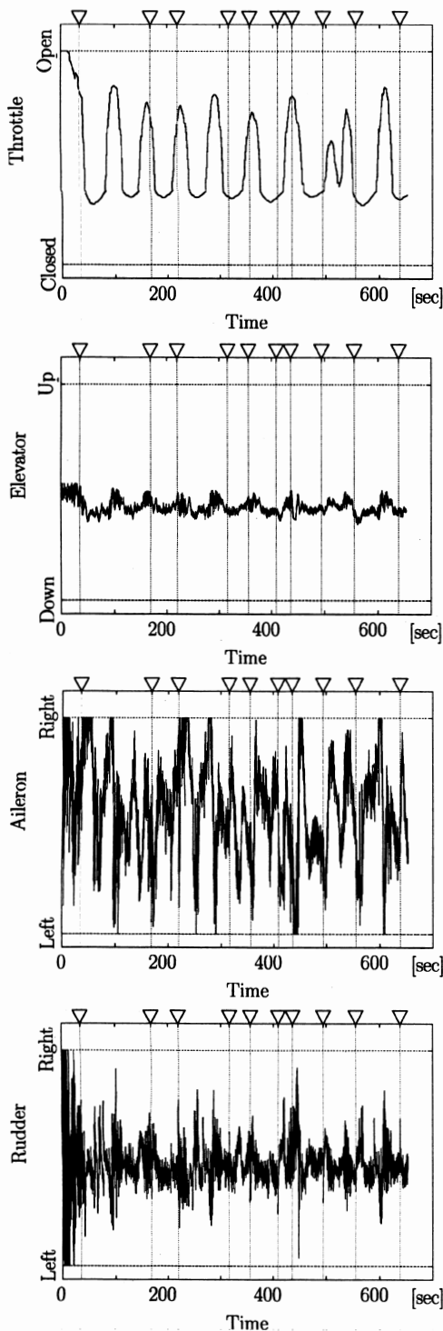
Fig. 11. Control inputs.
