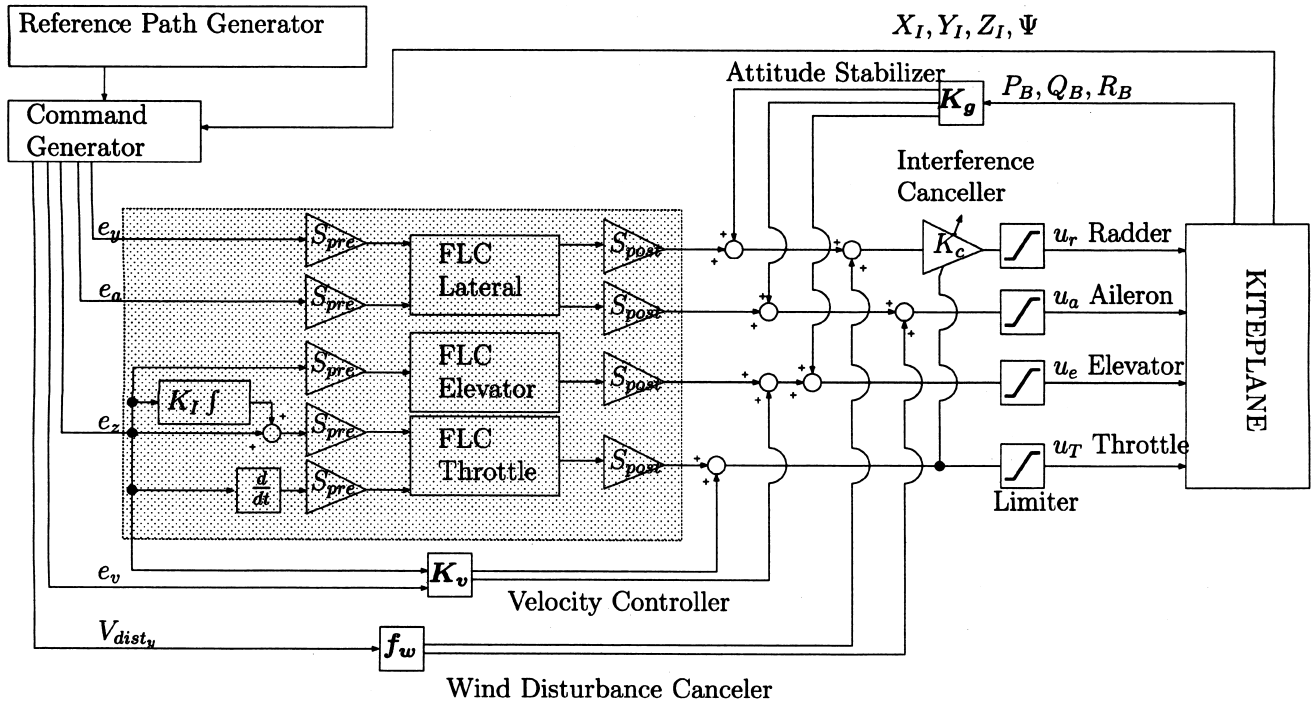
Fig. 6. Block diagram of the autopilot system.
