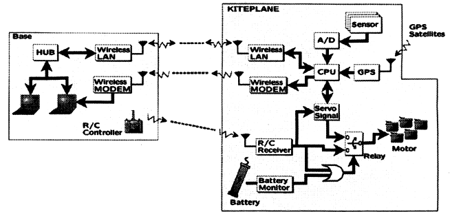
Fig. 2. Overview of the autopilot system.
