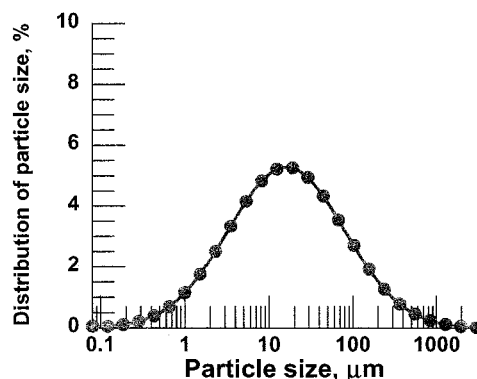
Fig. 4. Distribution of particle size of fly ash collected from a coal power plant against their size.
