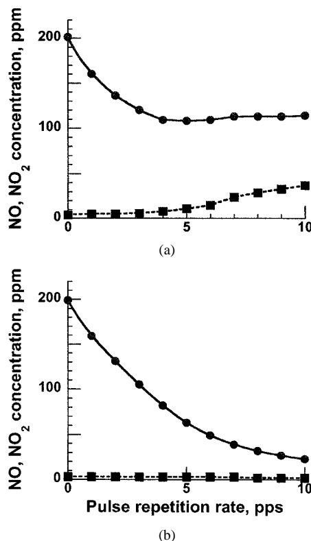
Fig. 8. As for Fig. 6 but with a mixture of N 2 (96.9%), NO (200 ppm) and H 2 O (3.1%): (a) without fly ash and (b) with fly ash (0.4 g/Nm 3 ). Other conditions of pressure and temperature were as in Fig. 6, ● NO, ■ NO 2 .
