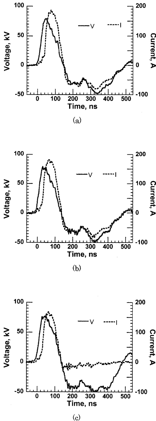
Fig. 5. Voltage and current waveforms for different gas mixtures. (a) N_2 , NO (200 ppm) without fly ash, (b) N_2 , NO (200 ppm) with fly ash ( 11.25 \text{ g/Nm}^3 ), and (c) N_2 , NO, O_2 (5%), H_2O (3.1%) and without fly ash. Condition, 1.01 \times 10^5 \text{ Pa} ; temperature 25 \pm 2 \text{ }^\circ\text{C} ; pulse rate 1 pps.
