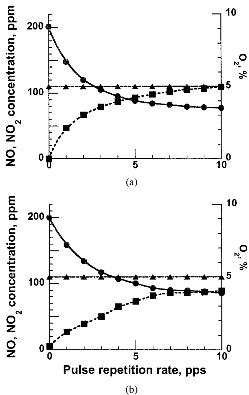
Fig. 7. As for Fig. 6 except the gas mixture was N 2 (95%), NO (200 ppm) and O 2 (5%): (a) without fly ash and (b) with fly ash (11.25 g/Nm 3 ). Other conditions of pressure and temperature were as in Fig. 6, ● NO, ■ NO 2 , ▲ O 2 .
