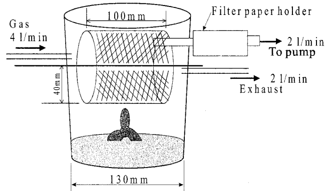
Fig. 2. Setup for measurements of the fly ash concentration.
