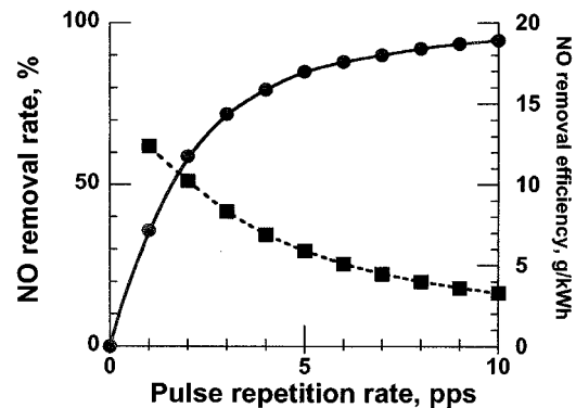
Fig. 11. NO removal rate (●) and NO removal energy efficiency (■) against pulse repetition rate in the presence of fly ash. Conditions are as in Fig. 10.
