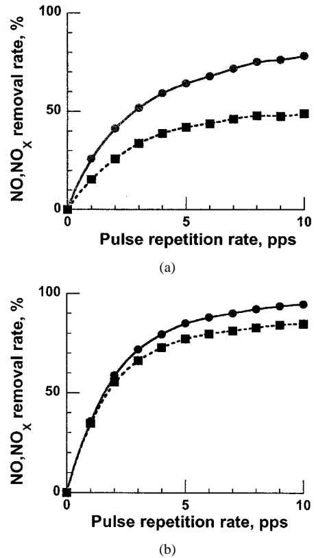
Fig. 10. Removal rates of NO and NO_x for a mixture of N_2 (91.9%), NO (200 ppm), O_2 (5%) and H_2O (3.1%): (a) without fly ash and (b) with fly ash ( 0.4 \text{ g/NM}^3 ). Other conditions of pressure and temperature were as in Fig. 6. ● NO, ■ NO_x .
