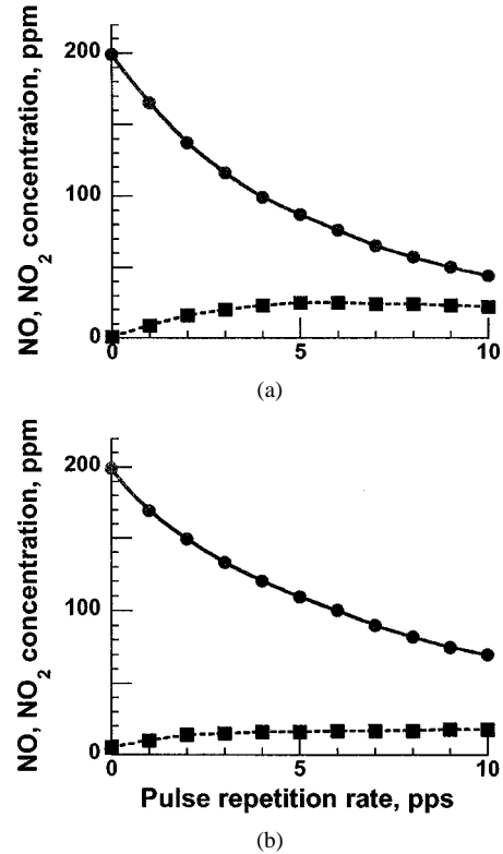
Fig. 6. Final concentration of NO and NO_2 . (a) Without the addition of fly ash and (b) with fly ash as a function of pulse repetition rate. Conditions: dry mixture of N_2 with initial NO concentrations of 200 ppm; fly ash, 11.25 \text{ g/Nm}^3 ; pressure, 1.01 \times 10^5 \text{ Pa} ; temperature 25 \pm 2 \text{ }^\circ\text{C} ; pulse width, 100 ns; peak voltage, 78.9 \pm 1.2 \text{ kV} ; peak current 173.5 \pm 7.5 \text{ A} , \bullet NO, \blacksquare NO_2 .
