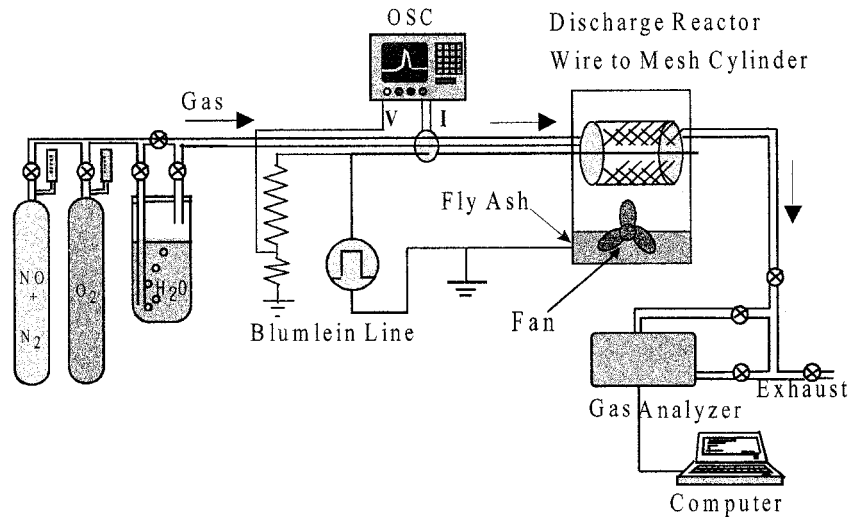
Fig. 1. Experimental setup for removal of NO in the presence of fly ash using a concentric coaxial reactor.
