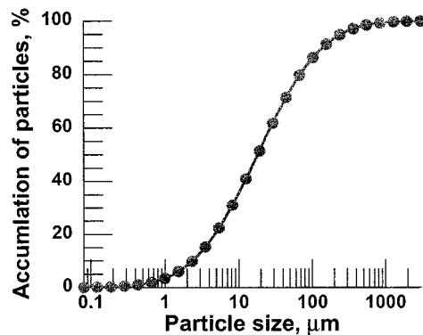
Fig. 3. Accumulation of particles of fly ash collected from a coal power plant against their size.
