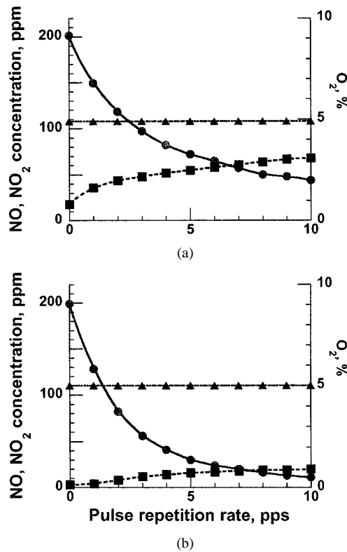
Fig. 9. As for Fig. 6 except the gas mixture was N_2 (91.9%) NO (200 ppm), O_2 (5%), and H_2O (3.1%): (a) without fly ash and (b) with fly ash ( 0.4 \text{ g/NM}^3 ). Other conditions of pressure and temperature were as in Fig. 6. ● NO, ■ NO_2 , ▲ O_2 .
