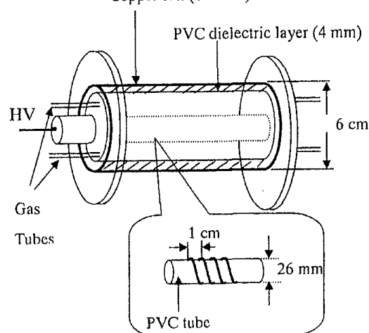
Figure 2. Discharge reactor configuration with a dielectric barrier. Wire diameter, 1 mm; reactor length, 1 m.
