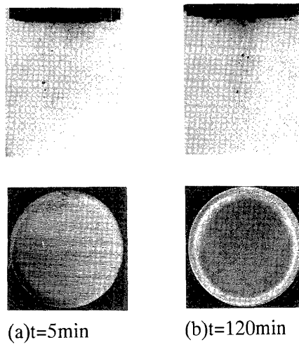
Fig. 9 Cavitation clouds and damage patterns in distilled water (pH0.7) (Carbon steel)
