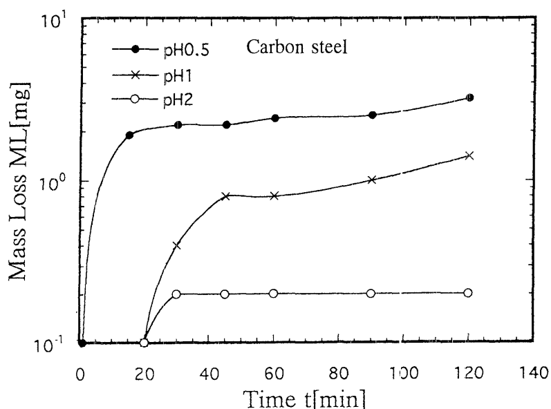
Fig. 4(b) Relation between mass loss ML by corrosion and test time t (Carbon steel)
