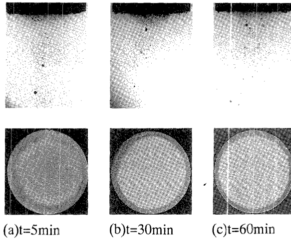
Fig. 6 Cavitation clouds and damage patterns in distilled water (pH7) (Aluminium)
