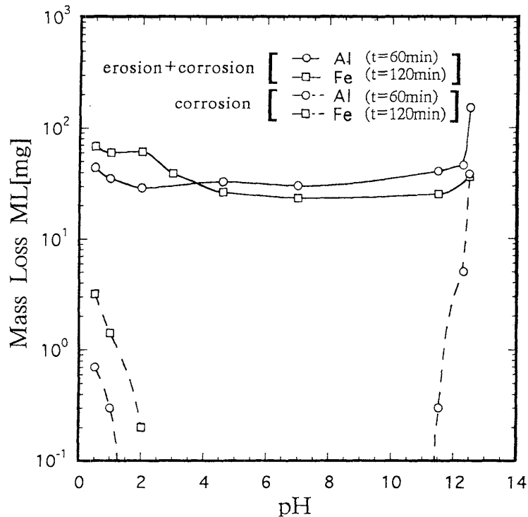
Fig. 5 Effect of pH on mass loss ML
