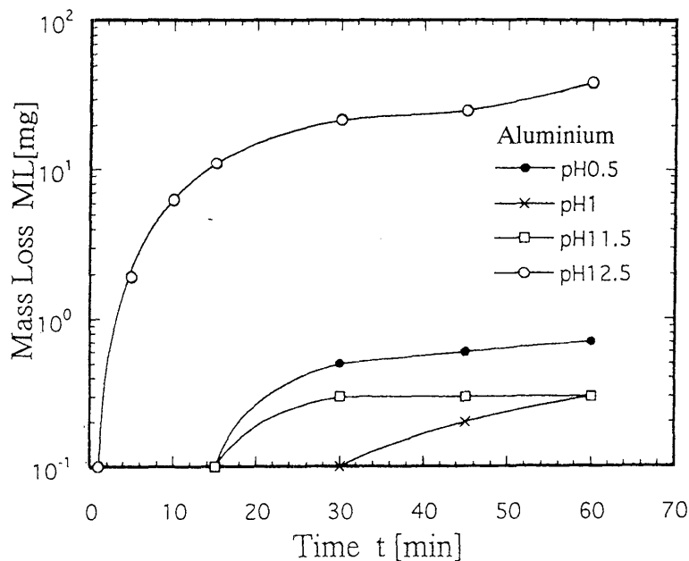
Fig. 4(a) Relation between mass loss ML by corrosion and test time t (Aluminium)
