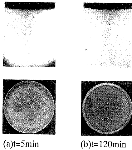
Fig. 10 Cavitation clouds and damage patterns in strong acid liquid (pH0.5) (Carbon steel)
