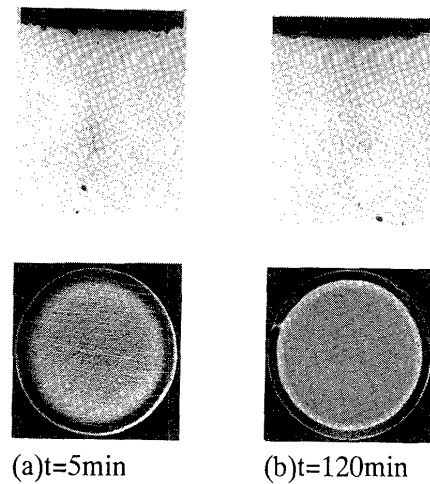
Fig. 11 Cavitation clouds and damage patterns in strong alkali liquid (pH12.5) (Carbon steel)
