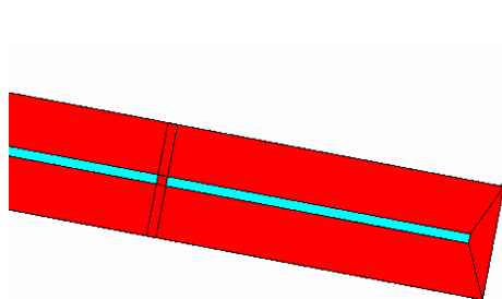
Figure 1 Dipole antenna printed on polyimide film.
