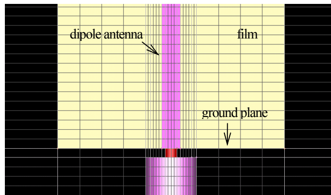
Figure 4 Modeling of antenna in Micro-Stripes
