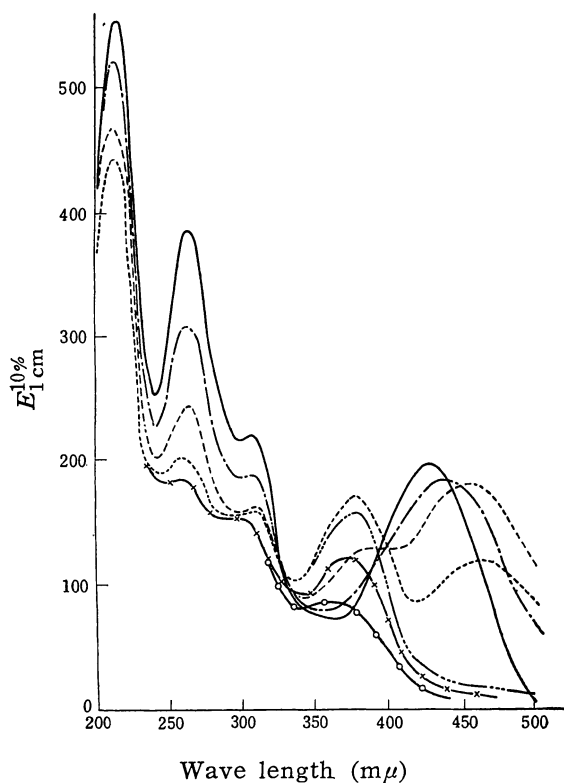
Fig. 3. Aq. luciferin solution (pH 5.6 phosphate buffer).
