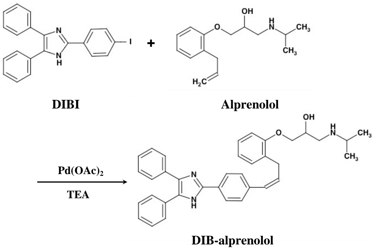
Fig. 1 Fluorescence labeling reaction of alprenolol with DIBI based on Mizoroki-Heck coupling reaction.
