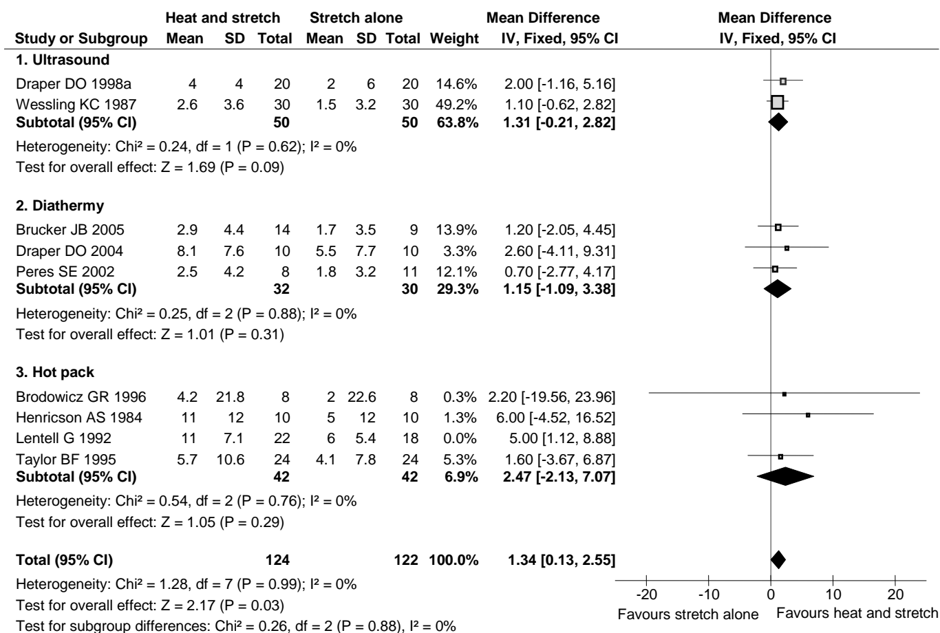
Figure 2. Forest plot of meta-analyses showing comparison of heat and stretch versus stretch alone measured after a single treatment according to method of heat application.
