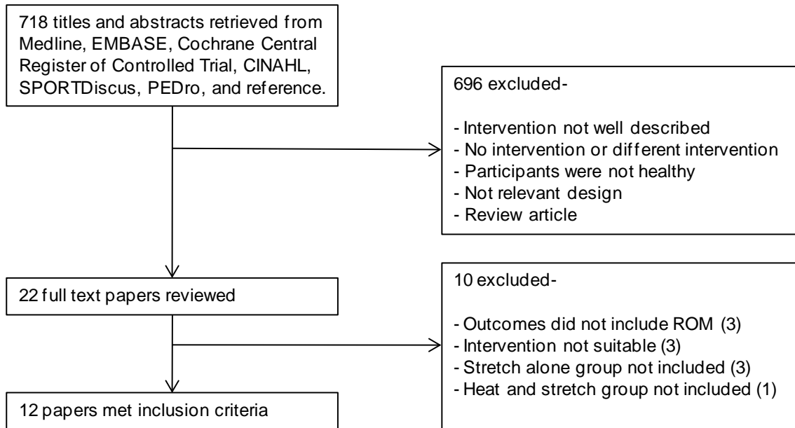
Figure 1. Flow chart with different phases of the search and selection of the studies included.
