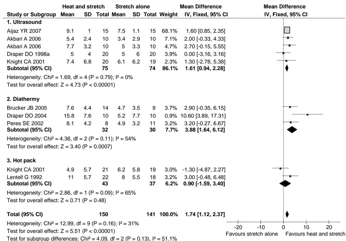
Figure 3. Forest plot of meta-analysis showing comparison of heat and stretch versus stretch alone measured after multiple treatments according to method of heat application.
