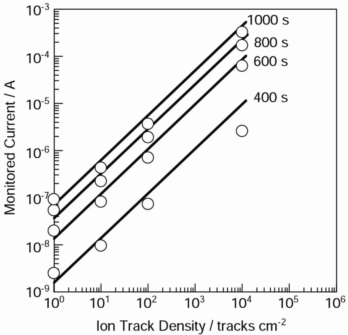
Fig.3 Linear relationship between heavy-ion-track density and monitored current for etching times of 400, 600, 800 and 1000 sec.
