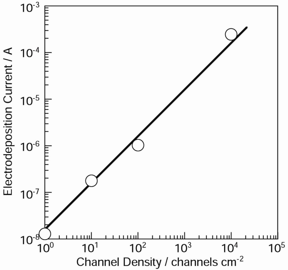
Fig.6 Relationship between channel density and cathodic current measured at a deposition time of 100 sec. Templates with a channel-diameter of (500±50) nm were used.
