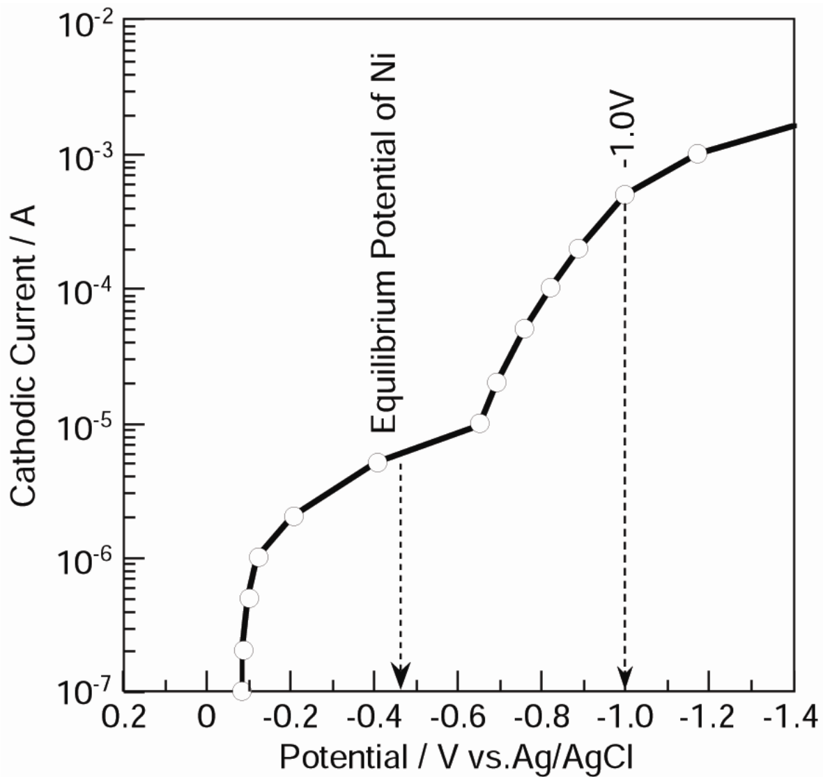
Fig.4 Cathodic polarization curve of a heavy-ion-track etched polycarbonate template with a channel-diameter of (500 \pm 50) nm and a channel-density of 10^4 channels \text{cm}^{-2} in a solution containing \text{Ni}^{2+} ions.
