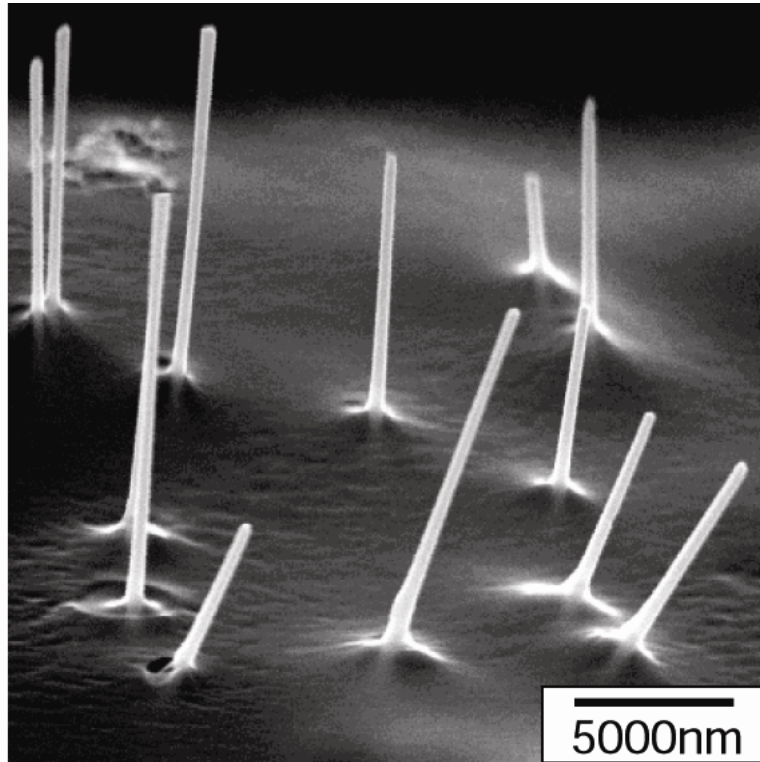
Fig.7 SEM image of Ni nanowires with diameters of (500\pm 50) nm and a channel-density of 10^4 channel \text{cm}^{-2} .
