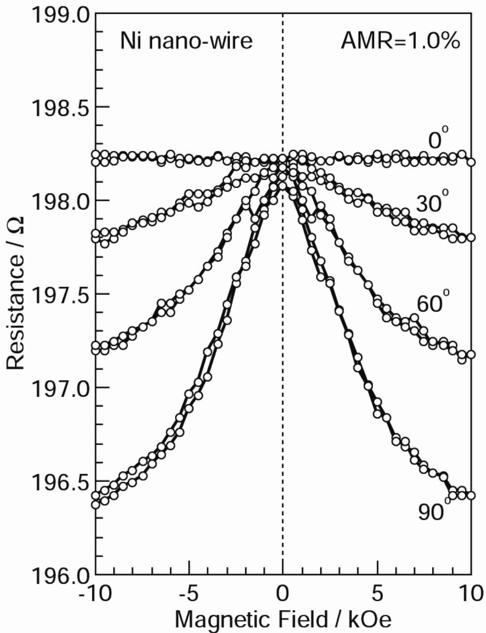
Fig.8 Magnetoresistive curves of a Ni nanowire electrodeposited into a heavy-ion-track etched polycarbonate template with a channel-diameter of (500 \pm 50) nm and a channel-density of 1 \text{ channel cm}^{-2} .
