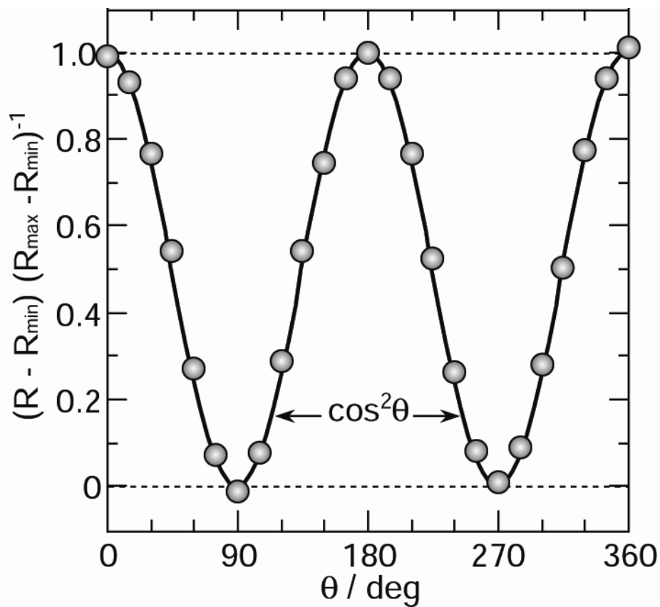
Fig.9 Angular dependence of the normalized resistance measured at a magnetic field of 10kOe of a single Ni nanowire electrodeposited into a heavy-ion-track etched polycarbonate template with a channel-diameter of (500 \pm 50) nm.
