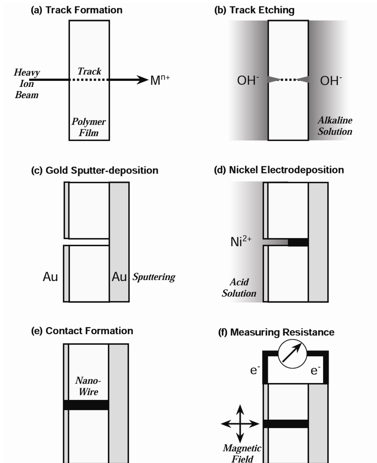
Fig.1 Fabrication and characterization of nanowires electrodeposited in a single-track nano-channel: (a) track formation, (b) track etching in alkaline solution, (c) sputter-deposition of gold layers on both sides of the membrane, (d) electrodeposition of a nanowire, (e) contacting the growing nanowire with the metal layer on the opposite side, (f) measuring the wire resistance as function of the applied magnetic field.
