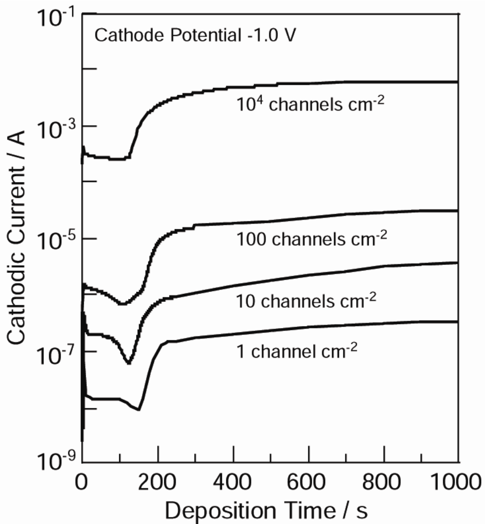
Fig.5 Effect of channel density on the cathodic current in a solution containing \text{Ni}^{2+} ions. Templates with channel-diameter of (500 \pm 50) nm were used.
