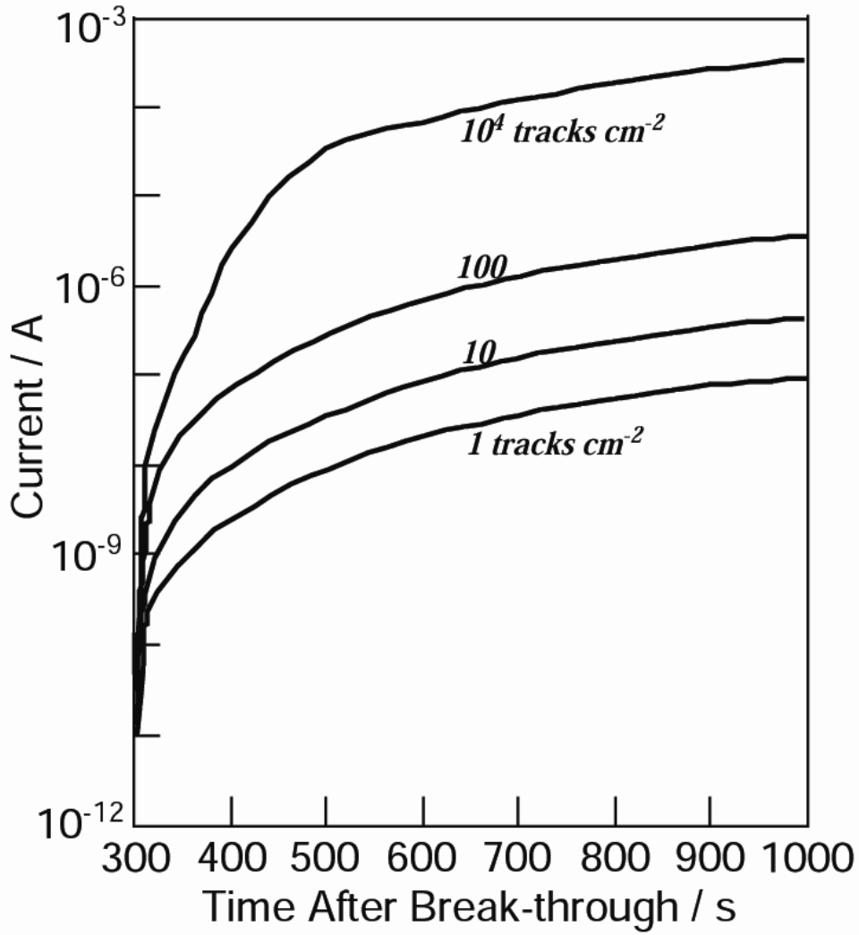
Fig.2 Time-dependence of current during track etching for samples with different heavy-ion-track densities (1, 10, 100 and 10^4 tracks \text{cm}^{-2} ).
