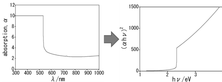
Figure 7. UV-VIS absorption spectra and (ahn)^2 vs. hn plot for determining the band gap energy of electrodeposited ZnTe.
