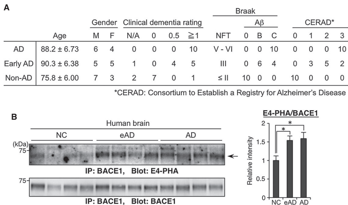
Figure 2. BACE1 is abnormally hyper-modified with bisecting GlcNAc in AD patients.
