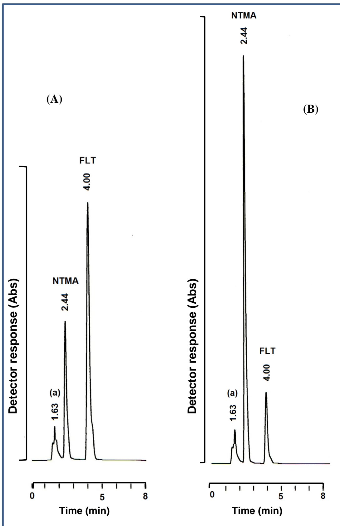
Fig. 1 Representative chromatograms for FLT (20.0 μg/mL) after exposure to (A) alkaline degradation (0.03 M NaOH at 90 °C for 30 min) and (B) acidic degradation (0.3 M HCl at 90 °C for 30 min), where: (a) is the solvent front, NTMA is 4-nitro-3-trifluoromethyl aniline (DP).
