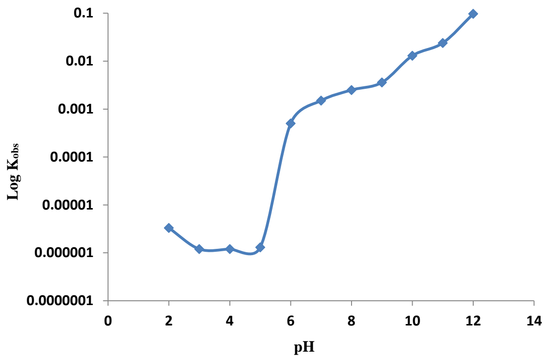
Fig. 4 pH-rate profile curve for FLT in BRB (0.04 M) at 100°C.
