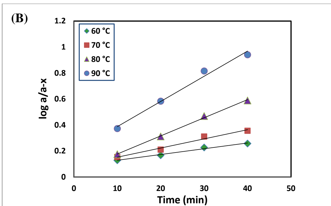
Fig. 2 Semi-logarithmic plots for the first-order degradation of FLT under (A) acidic (0.3 M HCl) and (B) alkaline (0.03 M NaOH) conditions at different temperature settings.
