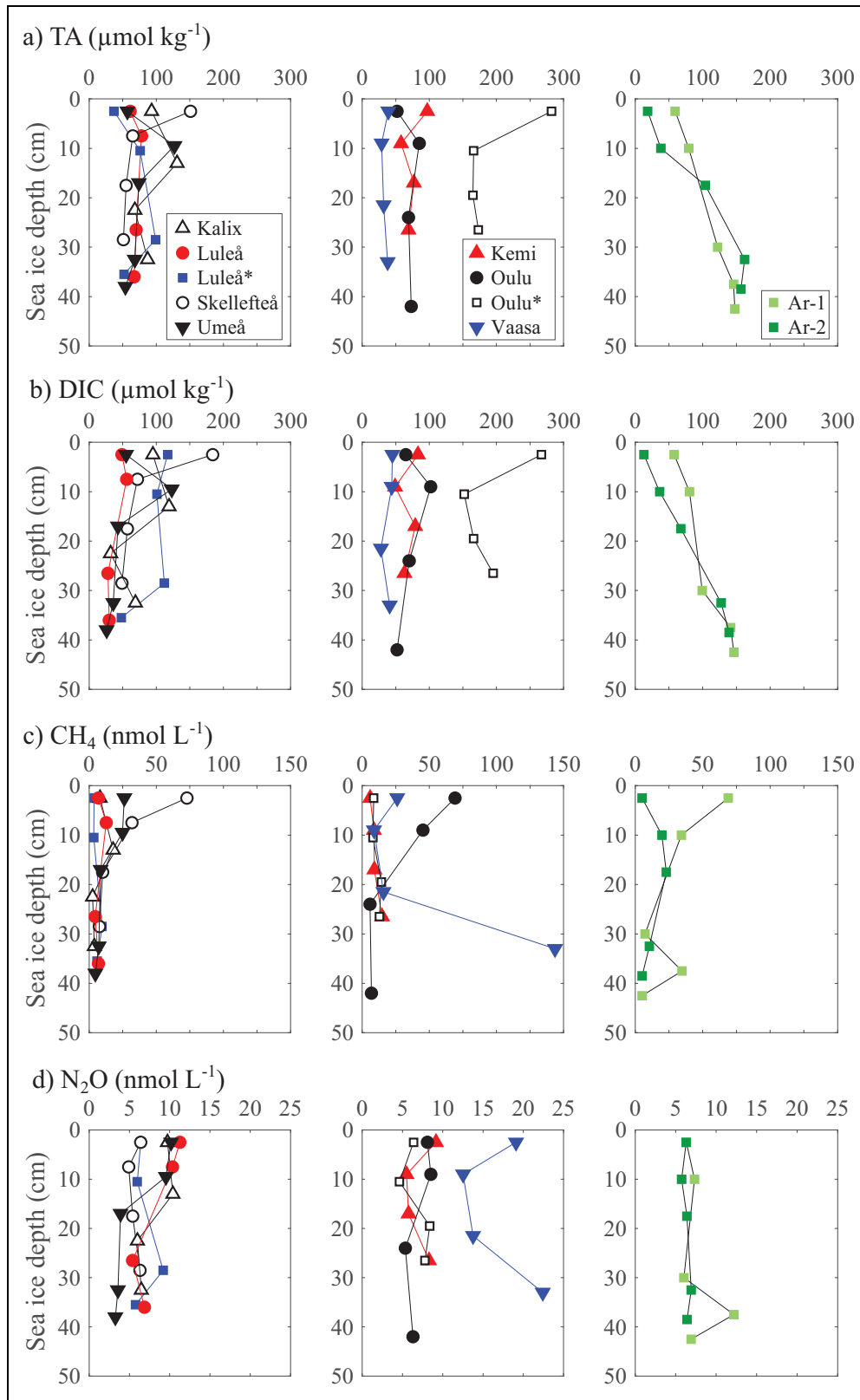
Figure 3. Sea ice profiles of total alkalinity, dissolved inorganic carbon, \text{CH}_4 , and \text{N}_2\text{O} concentrations. Data symbols are shape- and color-coded by station (locations in Figure 1 ) for (a) total alkalinity (TA, \mu\text{mol kg}^{-1} ), (b) dissolved inorganic carbon (DIC, \mu\text{mol kg}^{-1} ), (c) \text{CH}_4 ( \text{nmol L}^{-1} ), and (d) \text{N}_2\text{O} ( \text{nmol L}^{-1} ) concentrations. DOI: https://doi.org/10.1525/elementa.2021.00028.f3
