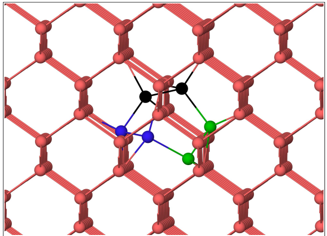
FIG. 6. A defect cluster found in molecular dynamics simulation of collision cascades with the mod-GAP interatomic potential. The cluster is comprised of a central vacancy and three dumbbell interstitials around it. The missing bond in the array of bonds at the center of the image can be helpful in locating the vacant site. Two of the dumbbells that surround the vacancy have [100] configuration (colored black and blue) and the third dumbbell is a [110]-type (green). Red atoms show the regular atomic sites in silicon lattice. All of the six atoms around the vacancy are 4-folded. The formation energy of the cluster is 5.57 eV according to DFT.
