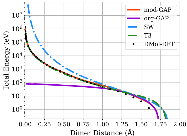
FIG. 3. The repulsive part of the SW, T3, org-GAP, and mod-GAP potentials.
