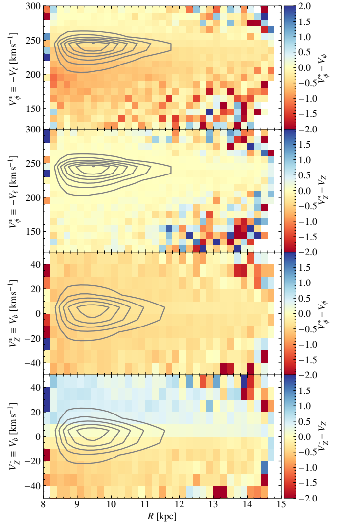
Fig. E.5. Error in the velocities for GOG when using our approximations (part 3). Median differences between V_\phi^* and V_\phi , and between V_Z^* and V_Z in bins in the R - V_\phi^* and R - V_Z^* projections.
