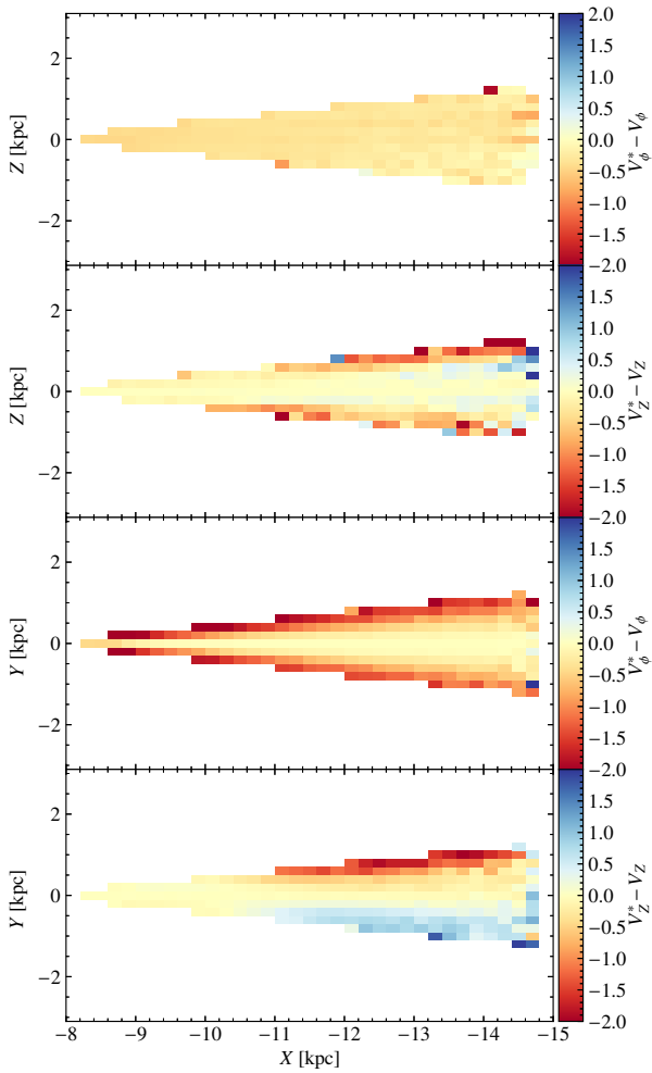
Fig. E.3. Error in the velocities for GOG when using our approximations. Median differences between V_\phi^* and V_\phi , and between V_Z^* and V_Z (Eqs. (4) and (5)) in bins in the X - Y and X - Z projections.
