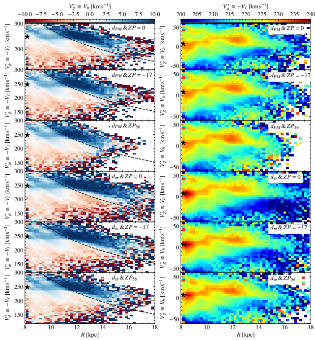
Fig. D.3. Phase space projections for different parallax zero point. The plot reproduces panels b and e of Fig. 14 using different distance estimations and parallax zero point as indicated in the legends. As explained in other parts of the article, the correction of the zero point combined with the different distance estimators used produce a change in the distance scale but in any case induces or removes the phase space substructure such as the one observed in this panels. The smallest distances are found when the Bayesian distances d_{PM} and the zero point ZP_{56} are used.
