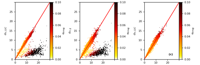
Fig. C.6. Red clump distance validation with the external catalogue L20. To enhance the illustration we use a larger RC sample here ( 147^\circ < l < 219^\circ and |b| < 30^\circ ). Panel a: comparison to L20 shows the presence of a population for which distances are overestimated using the K band. This is due to very high photometric errors (i.e. (e\_jmag) e\_kmag > 0.025 ). (b) Comparison between G and K band derived distances also highlights the same trend: K band distances are overestimated for poor photometry stars. (c) Replacing K band estimates with G where (e\_jmag) e\_kmag > 0.025 improves agreement with L20.
