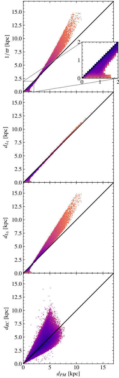
Fig. C.7. Comparison of the different distances used in this study. The comparison is done with respect to the d_{\text{PM}} distances. The discrepancies are small for small distances. For the case of the RC, we only compare stars with \varpi/\sigma_{\varpi} > 3 , since the rest of RC sources are not included in our set of d_{\text{PM}} . This is then misleading since for these stars the parallax retrieves better distances, but the real gain for the RC occurs exactly for the stars missing in this panel, in the regime where the photometric distances might be better than the ones from parallax alone. The peculiar shape shown in the inset of the top panel and present in the three top panels is composed of stars with large parallax error, for which the expectation values used in the d_{\text{PM}} estimation are larger than for instance the medians used in d_L .
