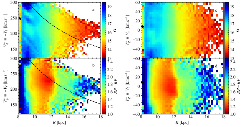
Fig. E.7. Photometry in different phase space projections. Median magnitudes G (top) and colour BP - RP (bottom) in the R-V_\phi^* plane (left) and R-V_Z^* plane (right) for the AC20- \omega/\sigma_\omega > 3 sample.
