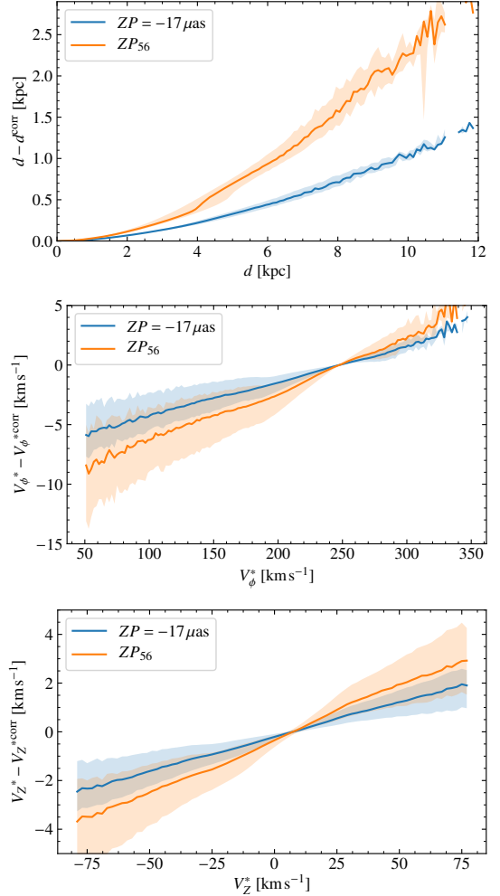
Fig. D.1. Effects of the zero point in parallax on distances and velocities. The comparison is done with respect to the case with the Bayesian distances d_{\text{PM}} where the zero point is not considered ( x axis) and the shaded areas show the percentiles 10 and 90 (i.e. they enclose 80% of stars). Top panel: we see how not correcting for the zero point produces overestimated distances. The zero point prescription ZP_{56} reduces even more the distances compared to the case of a fixed zero point ZP = -17 \mu\text{as} . The velocities ( middle and bottom ) scale linearly with the distance and thus we see the absolute magnitude of the velocities being larger when the zero point is not considered. We see null differences in the case of null proper motion, that is when the velocities equal that of the Local Standard of Rest.
