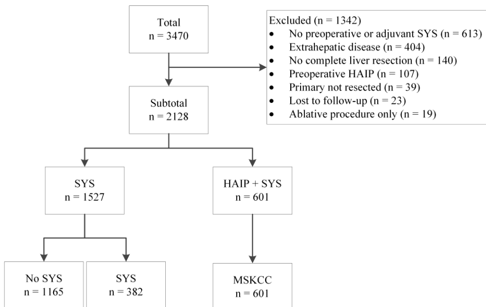
Figure 1. Study flowchart
