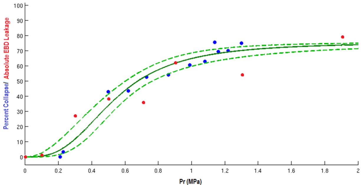
Figure 10.5: Overlay of experimental Pr-associated changes in vascular permeability with the percentage collapse of Definity ® . Blue dots represent the average in vitro collapse data and fitting of the collapse data with a logistic regression curve (solid green) with a 95% confidence interval (dashed green). Red dots indicate the average absolute vascular permeability from Chapter 7 to 9.
