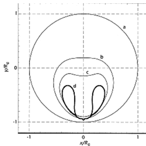
Figure 3.4: Asymmetric collapse profile of a microbubble near a semi-solid boundary. Reproduced from (Postema et al. 2004).
