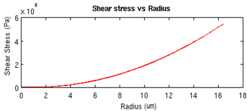
Figure 10.4: Shear stress as a function of radius. When Pr = 1.9 MPa a range of shear stresses are produced as the UCA grows and undergoes IC.
