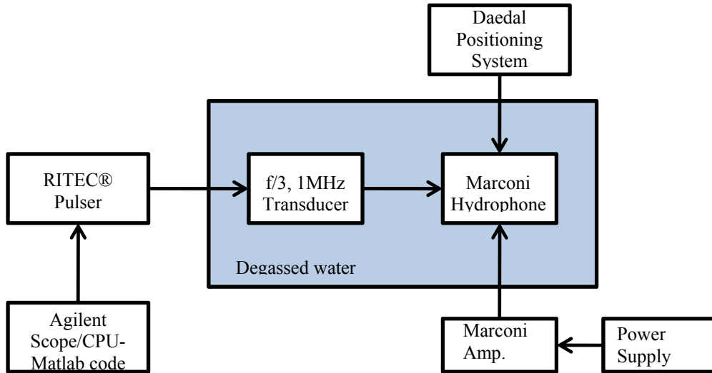
Figure 5.2: Calibration setup, including a pulser, transducer, hydrophone, amplifier, power supply and oscilloscope.
