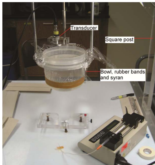
Figure 5.1: Experimental Setup
