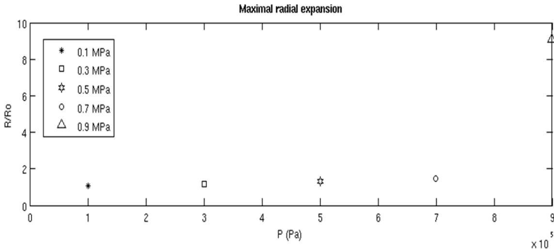
Figure 9.3: Maximal radial expansion of UCAs at varied Pr .
