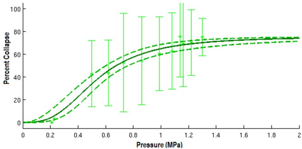
Figure 3.6: Percent collapse versus Pr: Definity ® inertial cavitation thresholds (MPa) at 1.0 MHz. (King et al. 2010).
