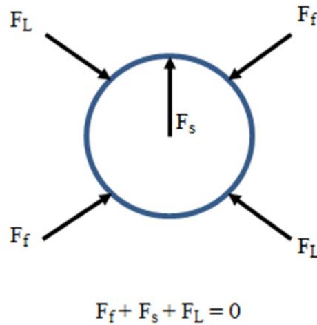
Figure 3.1: Forces acting at the bubble surface at equilibrium radius.
