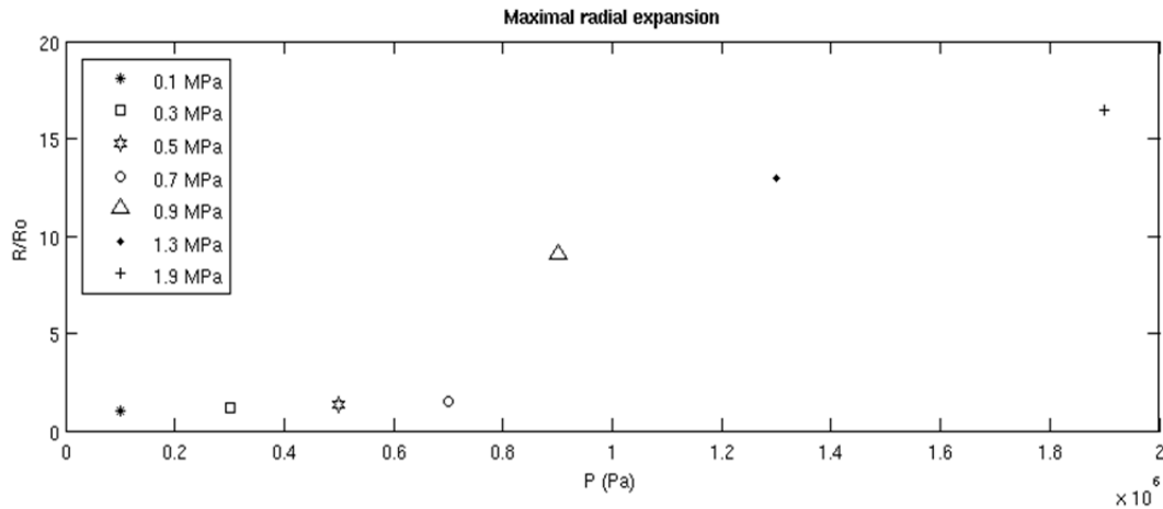
Figure 10.3: Maximal radial expansion for all experimental Pr, where a value of 1 means that maximal expansion is equal to the initial radius, ie. no expansion.
