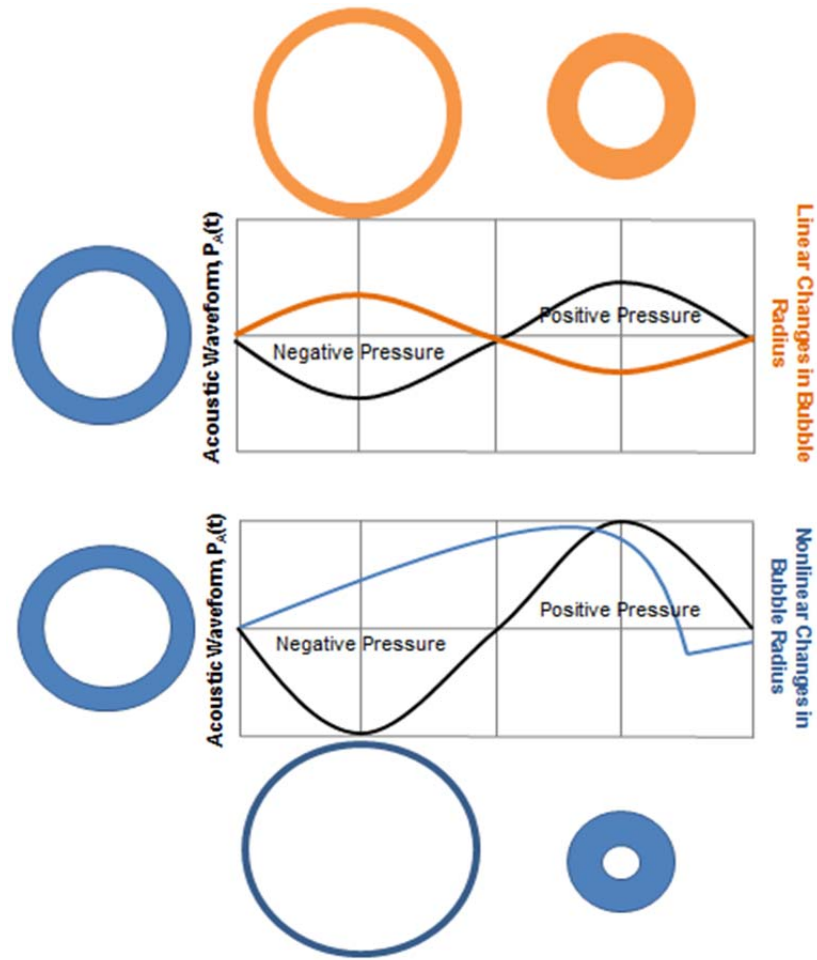
Figure 3.2: The changes in bubble radius with applied acoustic pressure. The linear case is valid when the acoustic amplitude is low, and the nonlinear case is for high amplitude waveforms, though only one waveform is depicted here.
