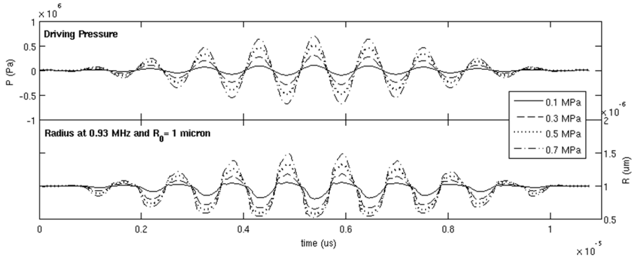
Figure 10.1: Radial displacement and driving pressure for low Pr.
