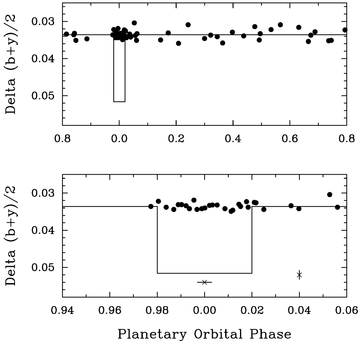
FIG. 1.— Top : Complete set of Strömgren \Delta(b + y)/2 differential magnitudes for HD 46375 plotted against orbital phase of the companion. The predicted depth and duration of the transit light curve are shown schematically. The star has no light variability on the planetary period larger than about 0.0001 mag or so. Bottom : Observations around the phase of predicted transit are replotted with an expanded scale on the abscissa. The horizontal error bar gives the uncertainty in the predicted time of midtransit. The vertical error bar indicates the precision of a single observation. Transits deeper than about 0.0001 mag are ruled out by these observations.
