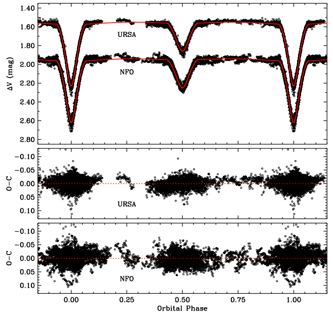
Figure 3. URSA and NFO observations of BT Vul along with our adopted light-curve model. The NFO photometry has been displaced vertically for clarity. Residuals in magnitude units are displayed at the bottom on an expanded scale.
