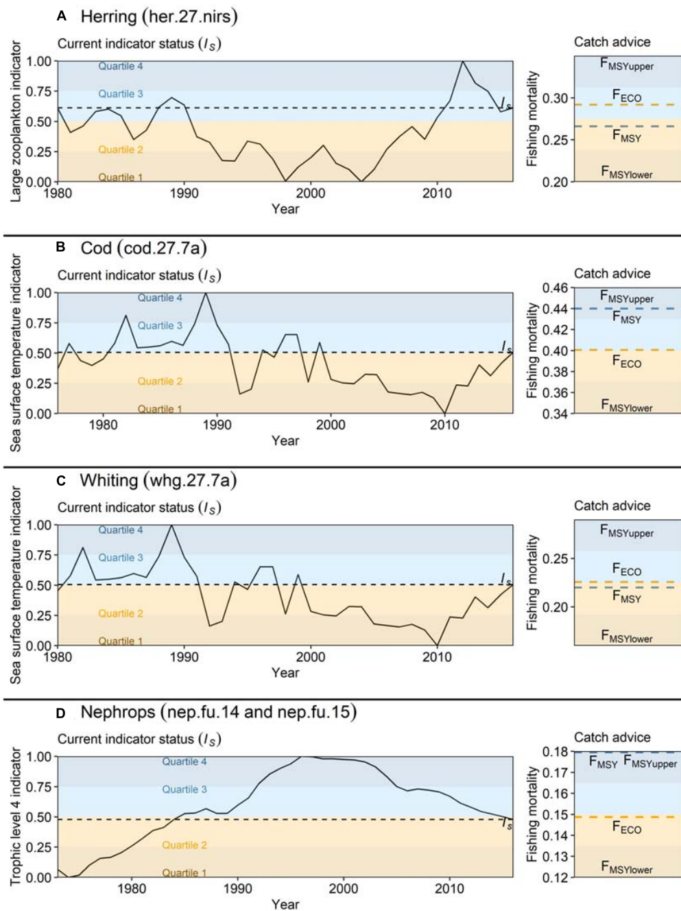
FIGURE 5 | From indicator to F_{ECO} . Examples are presented for Irish Sea (A) herring with large zooplankton biomass as an indicator, (B) cod with inverted sea surface temperature (SST; 3-year lag) as an indicator, (C) whiting with SST (3-year lag) as an indicator, and (D) Nephrops with the inverted biomass of trophic level 4+ as an indicator. On the left, all indicators are rescaled between zero and one to provide a percentile value which ranks the status of the indicator ( I_s ) in 2016 compared with previous years. On the right, the status of the indicator determines the placement of the F_{ECO} reference point within ICES F_{MSY} ranges.
