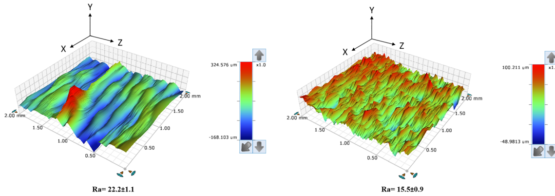
Fig. 9 3D topography profiles of specimen printing by a FFF process and b SLS process. Ra ( \mu\text{m} ) is the arithmetic mean surface roughness; it is by far the most commonly used parameter in surface finish measurement and for general quality control
