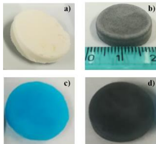
Figure 1: a) Cellulose and b) graphene-doped cellulose aerogel; c) cellulose and d) graphene-doped cellulose aerogel after Methylene-Blue absorption process.
