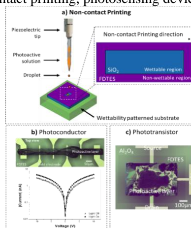
Figure 1: a) Schematic of the wettability assisted non-contact printing process to obtain micropatterned photoactive organic films and their integration into photosensing devices: b) photoconductors and c) phototransistors.
