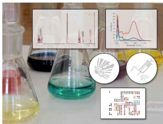
Figure 1 Background: dyes used in the CRIM-TRACK colorimetric sensor. Bottom right: Schematic representation of CRIM-TRACK colorimetric microchip. Middle right: Illicit substances symbols: explosives and controlled drugs. Top left: 1 H NMR spectra of dye (black line) and Hexamine-dye (Red line). Top right: UV Vis spectra of Hexamine (Blue line), dye (Black line) and Hexamine-dye mixture (Red line).
