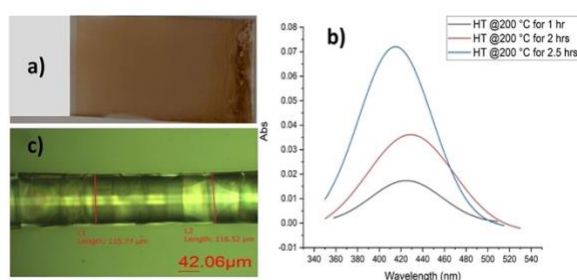
Figure 1: a) Silver nanoparticle/TEOS coating on a glass slide heat-treated at 200 °C for 2.5 hours; b) UV-Vis spectra of coated glass slides for samples heat-treated at 200 °C for 1, 2 and 2.5 hours, showing an absorption peak near 400nm, indicating the formation of silver nanoparticles; and c) Silver nanoparticle/TEOS coating on the core of an optical fibre.
