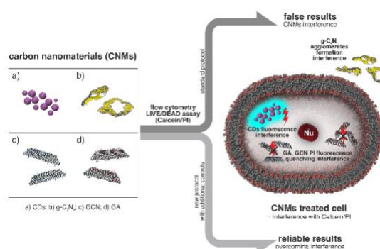
Figure 1: Illustration scheme of four types of emerging carbon nanomaterials (left) and various types of their interference with commercial dyes used in flow cytometry (right). Only by using our new approach with additional controls, it is possible to achieve reliable results of cell viability endpoint.
