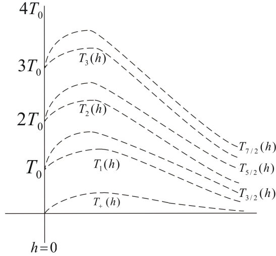
Figure 8.7: Simultaneous solutions to a boundary value problem with f(x) = x + \frac{1}{2}x^2 + \frac{1}{6}x^3 , A = 0 where the period annulus is unbounded.
