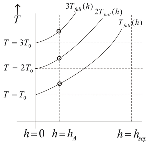
Figure 5.1: The limits of the full period functions nT_{full}(h) with n = 1, 2, 3 .
