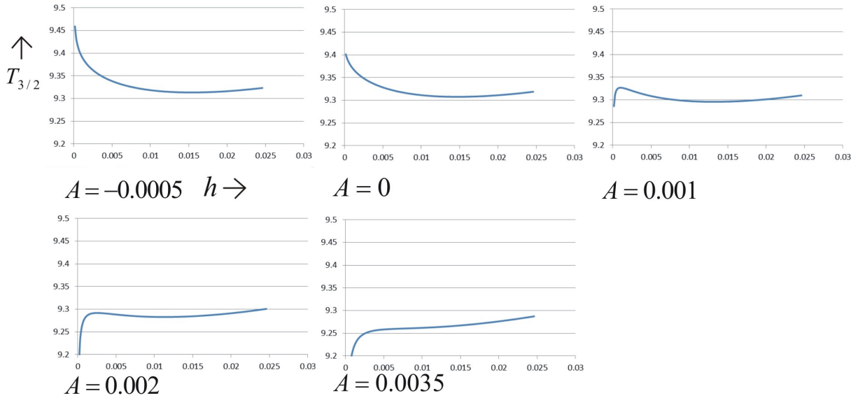
Figure 8.2: Numerical example for the mixed period function T_{3/2}^A for the quadratic Hamiltonian case f(x) = x(1 + x) while varying the parameter A . Five cases are shown for A . For A = -0.0005 and A = 0 only one local minimum occurs. For small positive A , i.e. A = 0.001 and A = 0.002 an additional local maximum occurs. For larger A , i.e. A = 0.0035 , the function is monotonically increasing and both local extreme points have disappeared.
