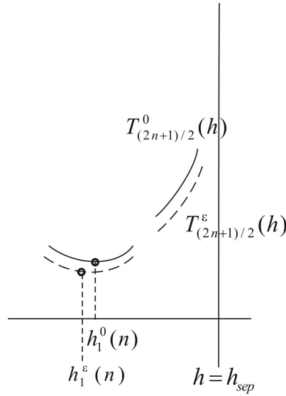
Figure 6.3: The persistence of a minimum h_1^\epsilon(n) for the mixed time-to-return functions T_{n+1/2}^A(h) for A = \epsilon > 0 in system (2.3) with real analytic f(x) satisfying conditions (1.3), (1.4), (1.5) and f''(0) > 0 .
