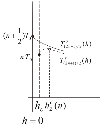
Figure 6.4: The creation of a maximum h_2^{\epsilon(n)} for the mixed time-to-return functions T_{n+1/2}^A(h) for A = \epsilon > 0 in system (2.3) with real analytic f(x) satisfying conditions (1.3), (1.4), (1.5) and f''(0) > 0 .
