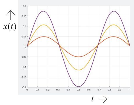
Figure 8.1: Numerical example of the co-existence of three solutions of type S_{3/2}^A to the boundary value problem for \lambda = 86.23908 , A = 0.002 for the quadratic Hamiltonian case f(x) = x(1 + x) . The initial conditions for the three solutions are \frac{dx(t)}{dt}|_{t=0} = 0.46 , \frac{dx(t)}{dt}|_{t=0} = 1.03 , \frac{dx(t)}{dt}|_{t=0} = 1.71 .
