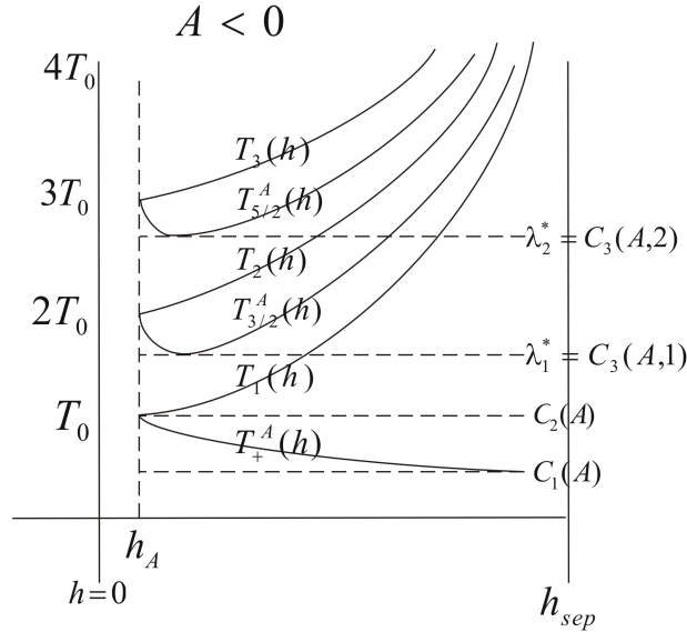
Figure 8.3: Conjectured time-to-return functions for simultaneous solutions to the boundary value problem for (2.3) with f(x) = x(1 + x) , x_s < A \leq 0 .
