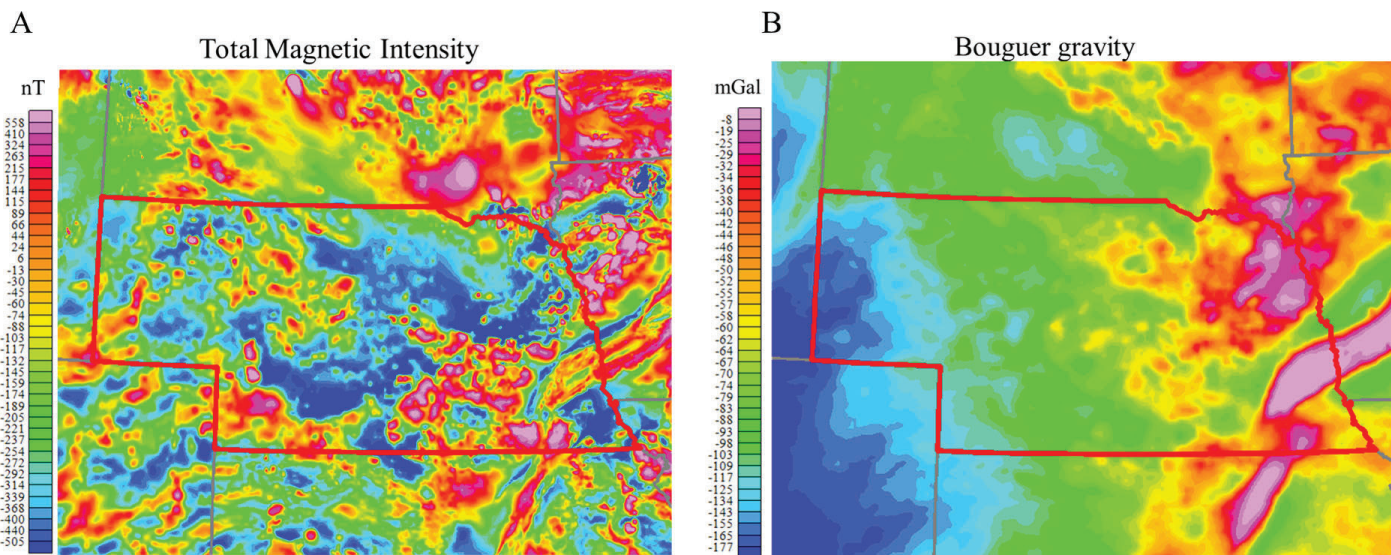
Figure 5. (A) Total magnetic intensity from Bankey et al. (2002), (B) Original Bouguer gravity from Kucks (1999).
