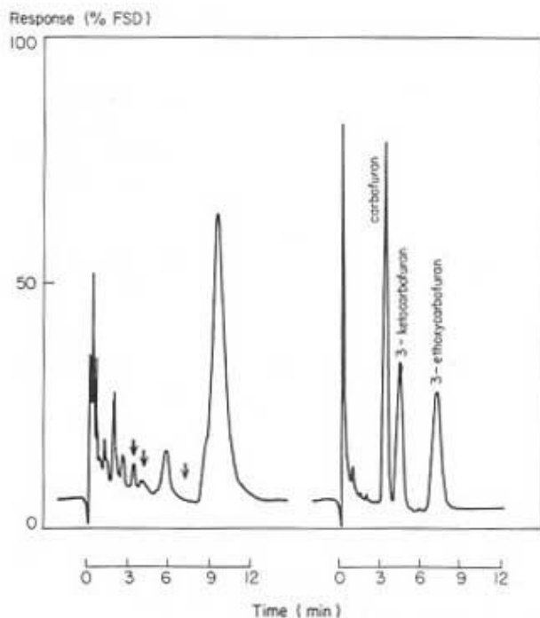
Fig. 1. Gas chromatograms with N-selective detector of (left) untreated rice stem extract, 19 mg of crop equivalent injected, and (right) 10 mg each of carbamate standards. Arrows indicate the retention times of carbamates determined.
