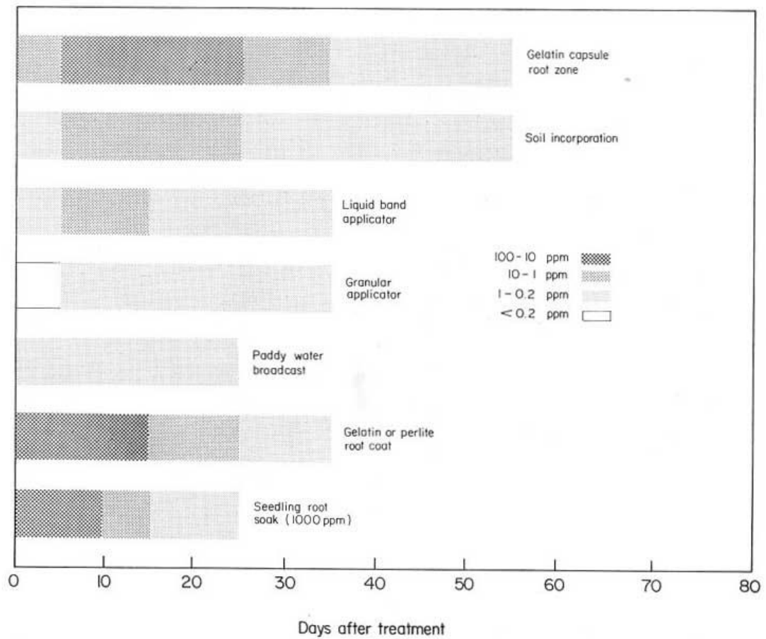
Fig. 5. Magnitude and duration of leaf residues of carbofuran from different treatments. Figures are estimates based on available residue data from rice treated in the field with 1 kg active ingredient/ha, except for seedling root-soak (0.15 kg active ingredient/ha). IRRI greenhouse, 1977.
