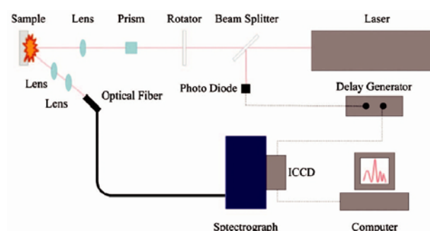
Figure 1. Schematic diagram of the experimental setup for LIBS measurements.
