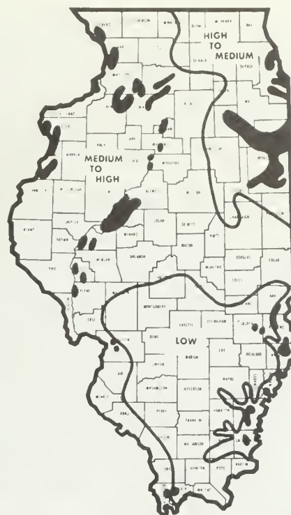
Potassium-supplying power. The black areas are sands with low potassium-supplying power. (Fig. 20)
