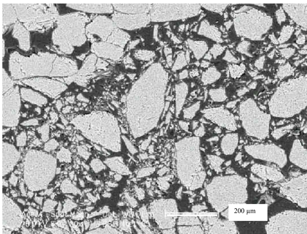
Fig. 16: Microphotographs of a shear band formed under 14 MPa of total confinement: (a) drained tests; (b) undrained test
