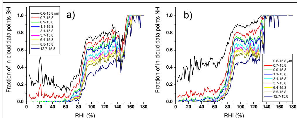
Fig. 4. Cloud presence fraction as function of relative humidity over ice for different crystal size thresholds as measured by the FSSP-300. If the probe, at a given RHI, observes any crystals having a size equal to or larger than the indicated thresholds found in the figure labels the data point is considered a cloudy data point. Data from SH (a) and from NH (b) .
