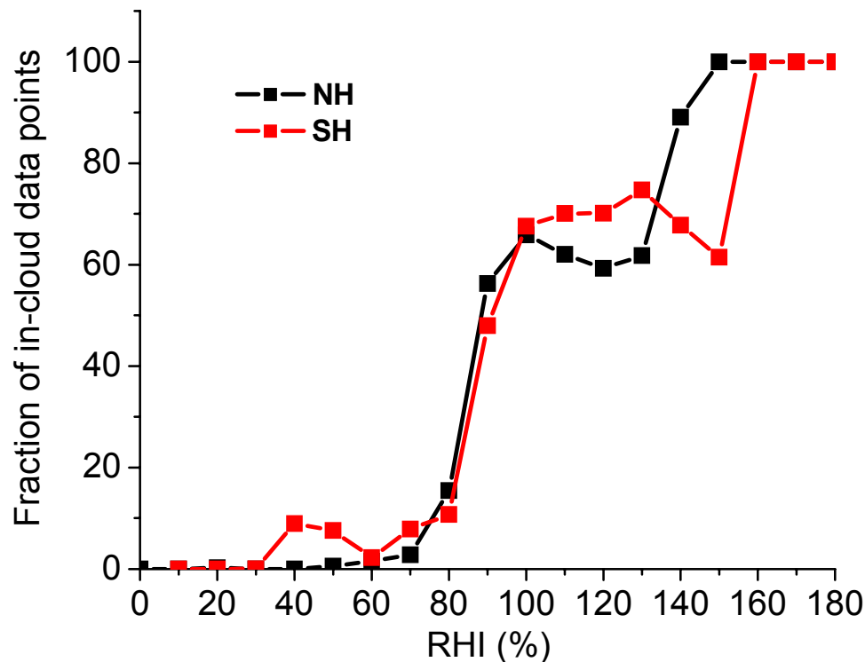
Fig. 6. Cloud presence fraction as a function of relative humidity over ice measured by the Polar Nephelometer. If the probe, at a given RHI, observes an extinction coefficient exceeding 0.05 \text{ km}^{-1} during four consecutive seconds the data point is considered a cloudy data point. Only data during straight and level flight segments are included.
