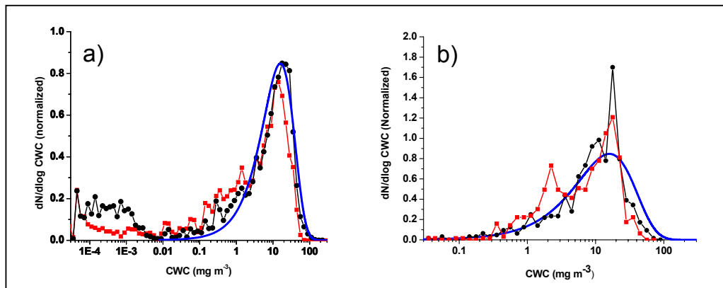
Fig. 10. Comparison between the observed distributions of cloud water content (SH red symbols and NH black symbols) and the distributions derived by using Eq. (5) and S_0 = 2 (blue line). In (a) all temperatures below 235 K and relative humidities between 95 and 105% RHI are used. In (b) the temperature only ranges between 225 and 227 K. The observed CWC is based on the sum of the FSSP-300 and 2D-probe. The derived distribution (blue line) is the same in both plots. Note the different axis scales.
