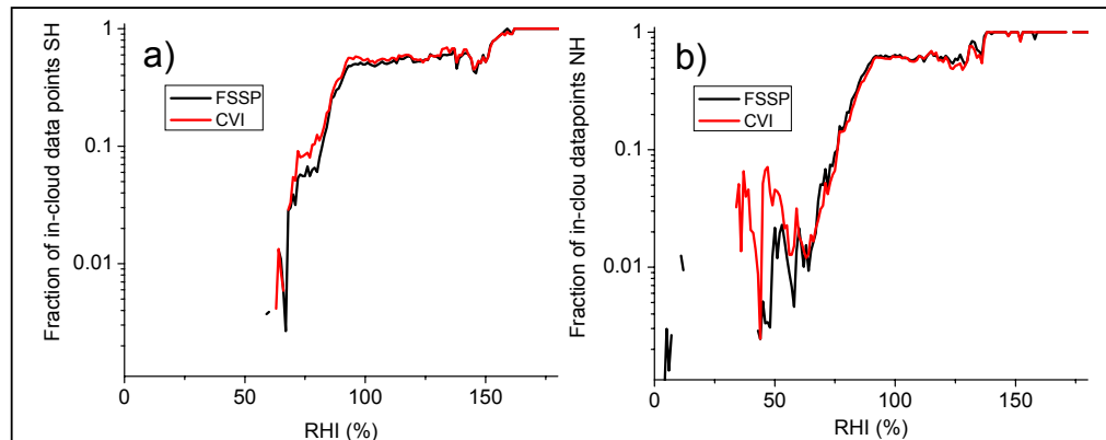
Fig. 2. Cloud presence fraction as function of relative humidity over ice using similar detection thresholds for the two probes with respect to crystal size ( > 4 \mu\text{m} ) and crystal number density ( > 0.3 \text{ cm}^{-3} ). Data from SH (a) and from NH (b).
