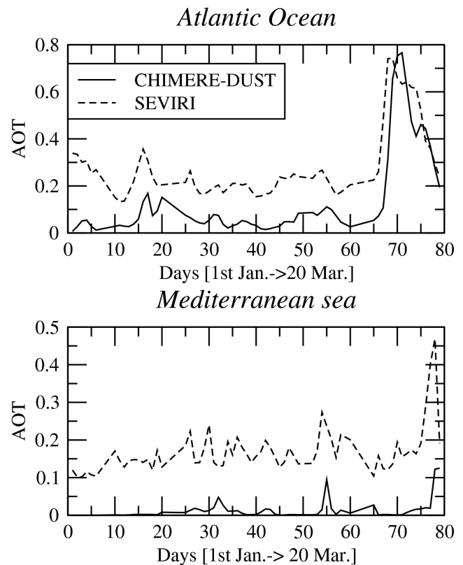
Figure 6. Comparison of aerosol optical thickness recorded by SEVIRI and modeled by CHIMERE-DUST during the first three months of 2006 and over two specific areas: Atlantic Ocean and Mediterranean Sea as displayed in Figure 3.
