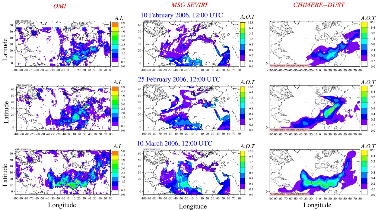
Figure 5. Maps of [left] aerosol index with OMI, [middle] optical thickness by SEVIRI and [right] modeled aerosol optical thickness, for the 10 February, 25 February and 10 March 2006 12:00 UTC.
