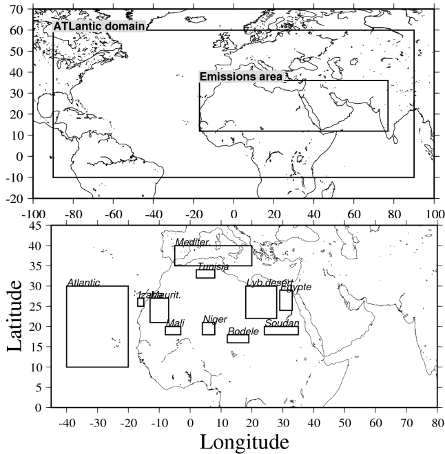
Figure 3. [top] Map of the CHIMERE-DUST simulation domains. The "ATL" domain used in this study extended from \lambda = -90^\circ W to \lambda = +90^\circ E and from \phi = -10^\circ S to \phi = +60^\circ N . The domain where the potential dust emissions are diagnosed is noted 'Emissions area'. [bottom] The selected areas used for comparisons.
