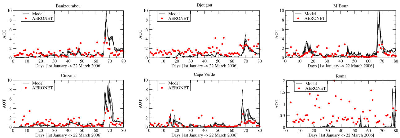
Figure 10. Time series of aerosol optical thicknesses modeled (all leads are superimposed) and recorded by the AERONET sunphotometers network (symbols) during the SOP0 period (from the 1st January to the 22 March 2006)
