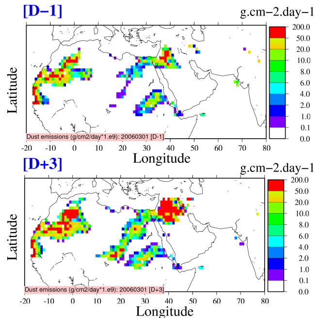
Figure 8. Daily integrated dust emissions fluxes ( \text{g}\cdot\text{cm}^{-2}\cdot\text{day}^{-1} ) from different leads ([D-1] and [D+3]) on 1st March 2006.
