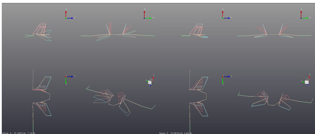
Figure 36: Measured FINAF F/A-18C Vertical Tail mode shapes (bending) around 15 Hz. Antimetric mode, 15.15 Hz (left) and symmetric mode, 15.66 Hz (right). Figure courtesy of VTT.
