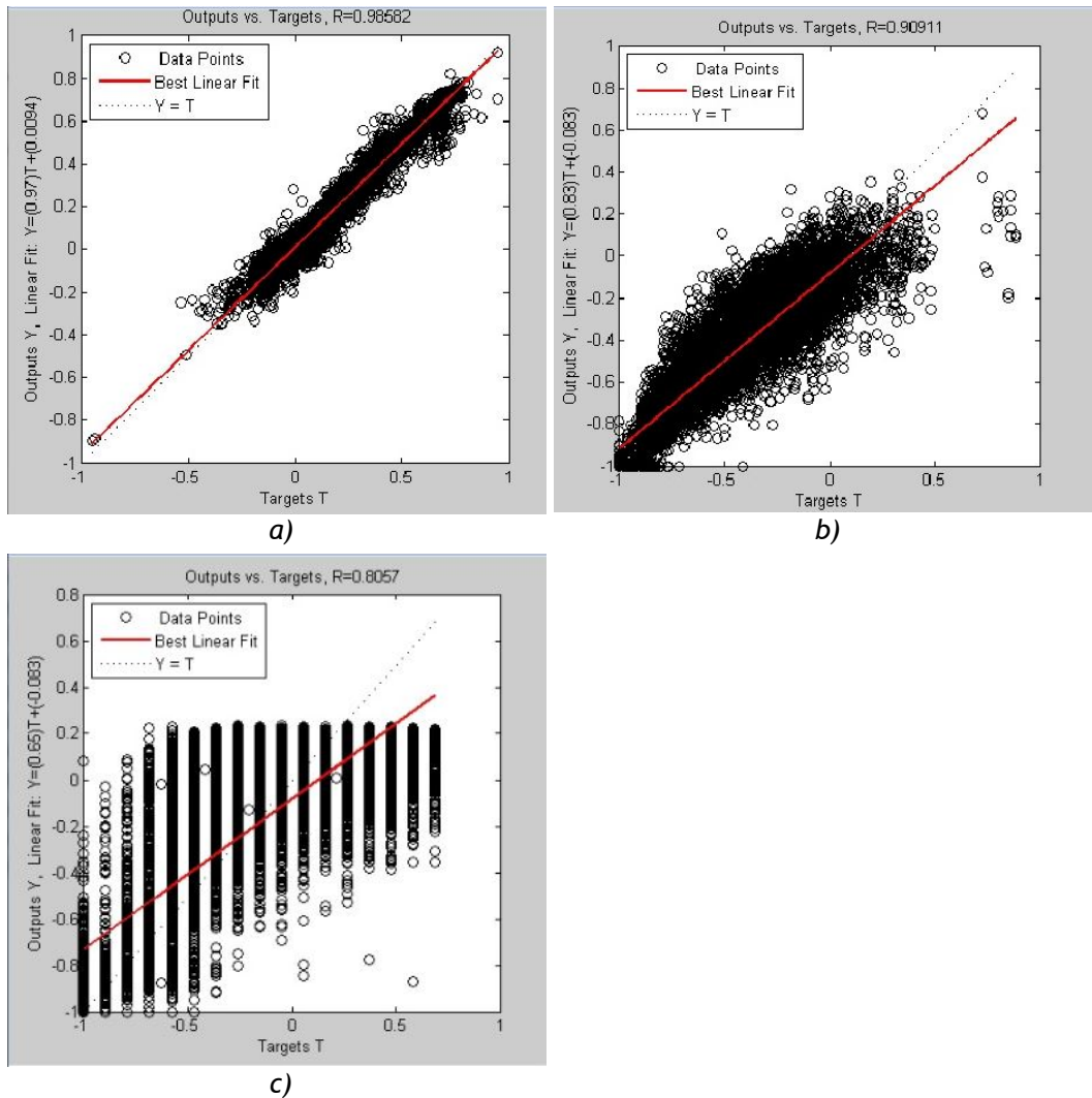
Figure 41: Subfigure a: Scatter of training static (low-pass filtered data) component (correlation 98,6%), b: amplitude component (correlation 91.0%), and frequency component (correlation 80.6%). Figure courtesy of Patria Aviation.
