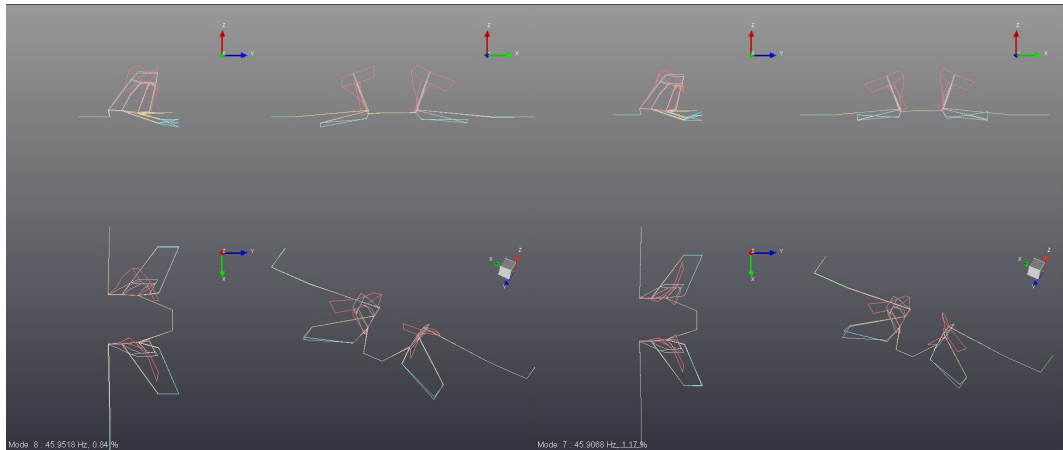
Figure 37: Measured FINAF F/A-18C Vertical Tail mode shapes (torsion) around 45 Hz. Antisymmetric mode, 45.95 Hz (left) and symmetric mode, 45.91 Hz (right). Figure courtesy of VTT.
