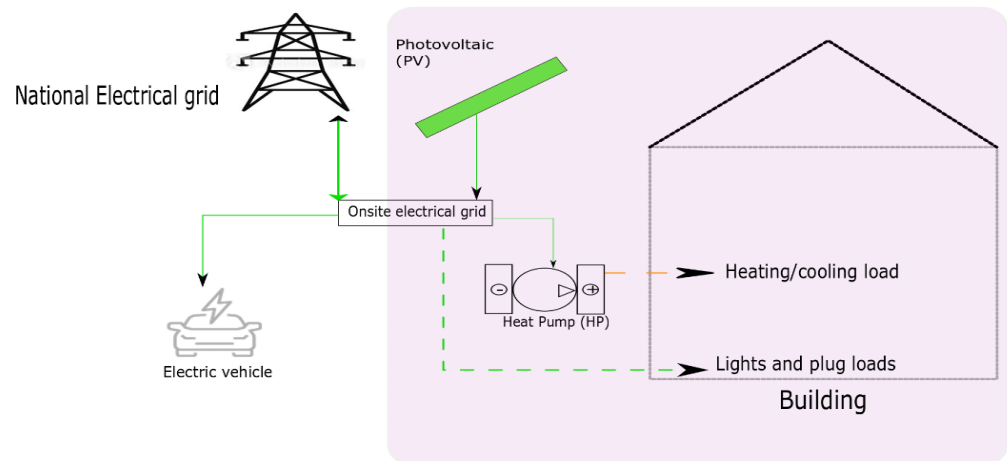
Figure 1. Main equipment installed on-site, heat paths (brown) and electricity paths (green) are shown.
