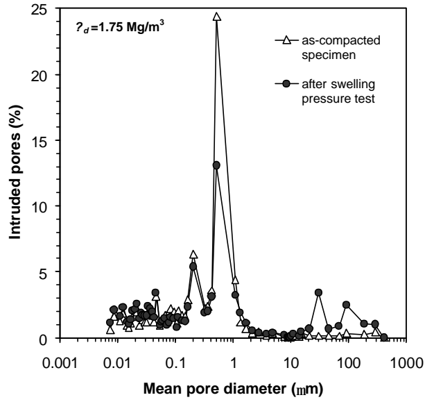
3 Figure 10. Pore-size distribution of as-compacted and wetted Compacted GMZ 4 bentonite; a) cumulated curve (b) derived curve
