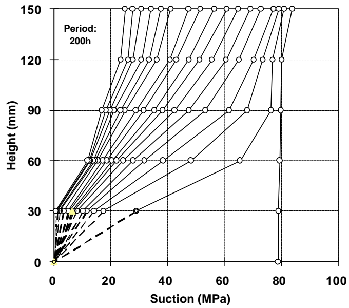
Figure 6. Suction profiles
