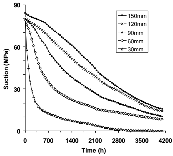
Figure 5. Evolution of suction during infiltration
