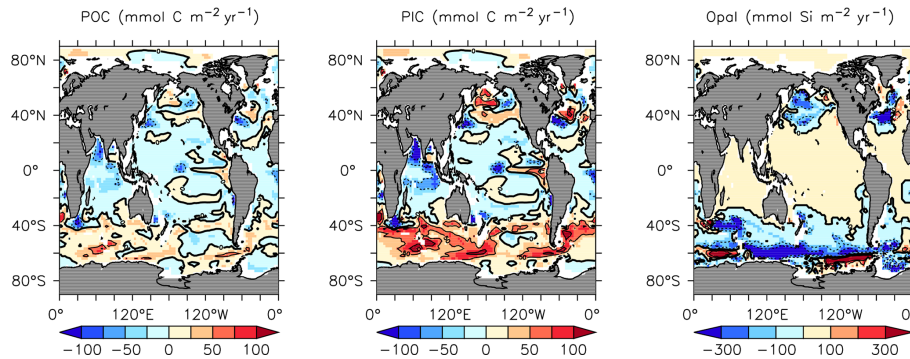
Figure 27. Modelled change in particle fluxes at 2 km depth, from 2014 to 2294.
