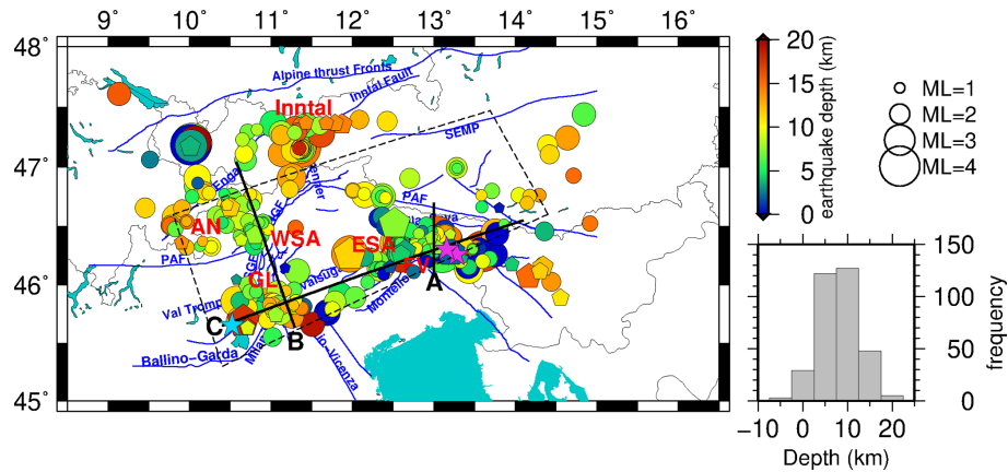
Figure 11. Distribution of the 335 well-located earthquakes in the target area after McMC inversion (single-event mode). Circles are earthquakes that were incorporated in the simultaneous inversion, and pentagons are 43 additional earthquakes with fewer picks. The color and size of the circles indicate the depth and magnitude of the earthquakes, respectively (magnitude is taken from national catalogs). The dashed black box indicates the periphery of the SWATH-D network. Purple stars show the location of Friuli earthquake of 6 May 1976 ( M_L 6.4) and its major aftershock on 15 September 1976 ( M_L 6.1) (Slejko, 2018), and the blue star is the Salò earthquake on 24 November 2004 ( M_L 5.2; Viganò et al., 2015). Black lines indicate cross sections shown in Fig. 12. Faults are compiled from geological maps of the Italian geological survey, including Avanzini et al. (2010); Bartolomei et al. (1967); Bosellini et al. (1967); Braga et al. (1971); Castellarin et al. (1968, 2005); and Dal Piaz et al. (2007) and complemented by fault traces published in Handy et al. (2010) and Schmid et al. (2004, 2008). Abbreviations are as follows: ESA stands for eastern southern Alps, WSA stands for western southern Alps, FV stands for Friuli-Venetia region, GL stands for Giudicarie–Lessini region, AN stands for Austroalpine nappes, PAF stands for Periadriatic Fault, NGF stands for northern Giudicarie Fault, SGF stands for southern Giudicarie Fault. The histogram on the right side indicates the depth distribution of the earthquakes in the crust.
