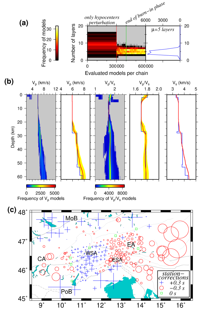
Figure 9. (a) On the left histogram, the probability of the number of layers of the random models introduced by Markov chains during the evolution are shown (color indicates number of models). On the right histogram, the number of layers of the models after burn-in phase is given. (b) V_P , V_P/V_S , and V_S models after MCMC simultaneous inversion. Figure characteristics are similar to Fig. 7. The velocity models are recovered down to \sim 63 km depth. (c) P wave station corrections of all the stations that were involved in the inversion corresponding to the 1-D velocity model in (b). Negative corrections (red circles) indicate earlier arrivals (indicative for higher velocities in the shallow subsurface) and positive corrections (blue crosses) indicate delayed arrivals (representative for lower velocities underneath the station). The faults are same as in Fig. 2. Abbreviations are as follows: CA stands for central Alps, EA stands for eastern Alps, ESA stands for eastern southern Alps, WSA stands for Western Southern Alps, MoB stands for Molasse Basin, and PoB stands for Po Basin.
