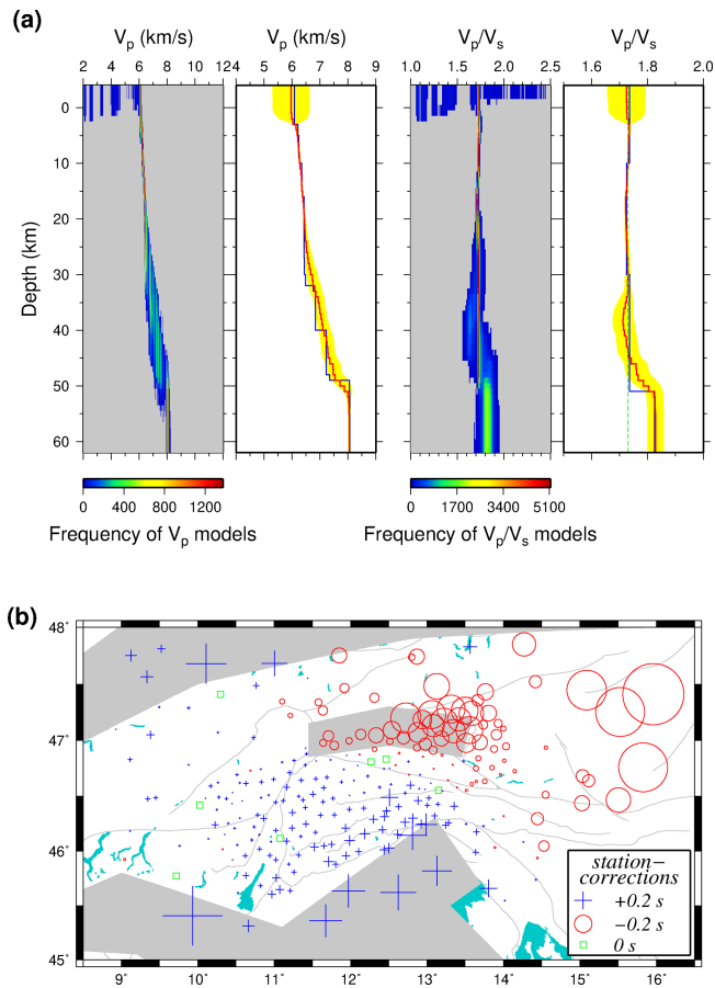
Figure 7. (a) Recovery of the V_p and V_p/V_s models after the synthetic test. The results are shown with heat maps (probability histogram vs. depth; warm and cold colors correspond to higher and lower probabilities, respectively) with gray areas showing zones with no model achievement. The modified average model (solid red line), most probable model (solid blue line), and corresponding uncertainty of 1\sigma (yellow zone) for both V_p and V_p/V_s models are shown as well. The V_p/V_s ratio of \sqrt{3} is displayed with the dashed green line. (b) Recovered P wave station corrections of all the stations that were involved in the MCMC inversion. Blue crosses show positive values reflecting lower velocities, and red circles display negative values indicating higher velocities than expected. Regions indicated in gray have shallow high- or low-velocity anomalies (see Fig. 5 for more information). Symbol size corresponds to correction amplitude. The faults are same as Fig. 2.
