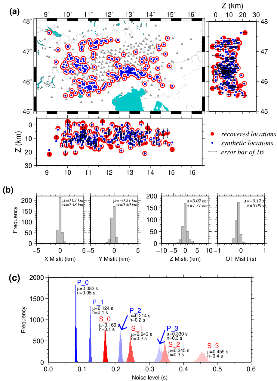
Figure 6. (a) Recovery of the hypocenters after synthetic test. Red circles are recovered earthquakes with a 1\sigma error bar (error bars of latitude and longitude are invisible at this scale), and blue dots are the synthetic locations. The gray triangles show the stations. (b) Histograms of the misfit between recovered hypocenters and original ones. The hypocenters are recovered very well, with an average misfit of 20 m ( \pm 380 m) in longitude, 210 m ( \pm 400 m) in latitude, 110 m ( \pm 1.131 km) in depth, and 0.12 s ( \pm 0.08 s) in origin time. (c) The recovered noise levels after MCMC for individual pick types and quality classes are slightly higher than the random noise, which was added to the synthetic travel time data.
