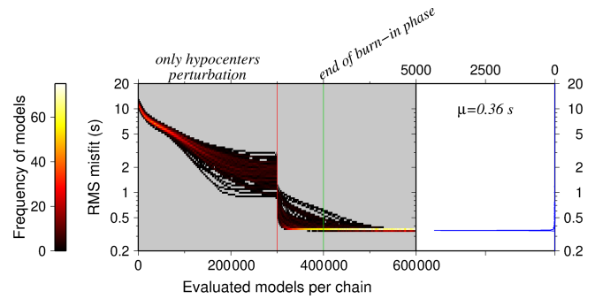
Figure 8. On the left histogram, the rms misfit along Markov chains during the inversion evolution is shown (color indicates number of models; please see color palette table on the left). Before the red line (300 000 models), only the hypocenters are perturbed and beyond that the V_p , V_p/V_s ratio, station corrections, and noise levels are allowed to change as well. The green line indicates the end of the burn-in phase after \sim 400\,000 models. On the right histogram, the rms misfit for all the models after burn-in phase is shown. The best-fitting models are characterized by an average 0.36\text{ s} rms misfit.
