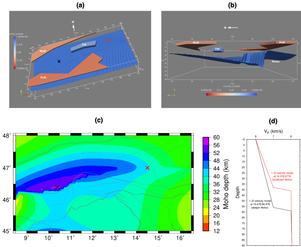
Figure 5. The 3-D synthetic V_p velocity model. The V_p/V_s ratio was fixed to \sqrt{3} in the entire model. (a) and (b) Contours of the Moho and shallow anomalies of the PoB, MoB, and TW from different view directions. (c) Modified Moho depth map based on Spada et al. (2013). (d) A 1-D velocity model of two different locations with shallower and deeper Moho retrieved from the 3-D synthetic velocity model (the locations are shown with red and black crosses in (a) and (c), respectively). The faults are the same as those in Fig. 2.
