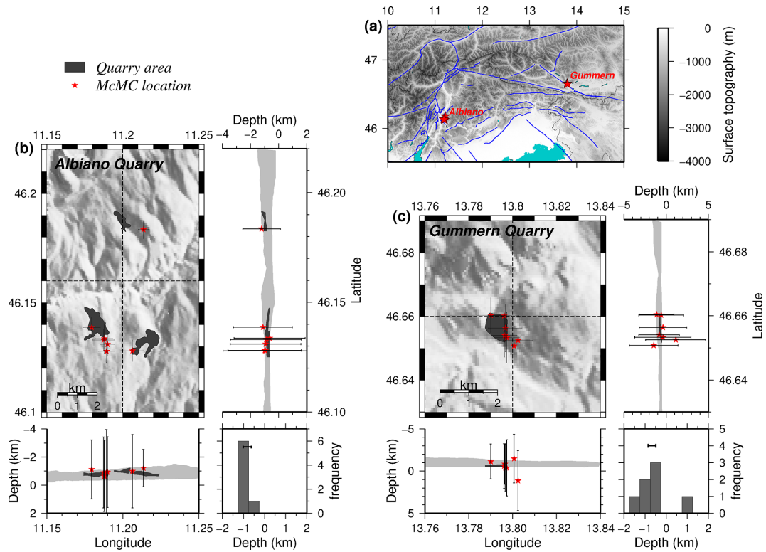
Figure 10. (a) Map view showing the location of quarry blasts relocated using single-event mode of McMC, with solutions of the 1-D velocity model and station corrections from the simultaneous inversion of earthquakes. (b) and (c) Epicenter and depth distribution of the blasts associated with two quarries close to Albiano in Italy and Gummern in Austria, respectively. The light gray band in the cross sections shows the surface elevation variation within the map view boundary. The dark gray zones show the location and surface elevations of the quarries. The depth histogram is also shown for each quarry (the bar in the depth histograms displays the surface elevation within the quarry area). Please note that elevations above the sea level are shown with negative values.
