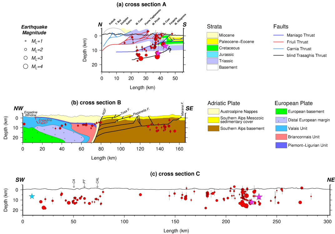
Figure 12. Seismicity distribution in depth along three profiles of A, B, and C in Fig. 11. For better clarity, the depth and length scales of cross section A are magnified by a factor of 1.5 (without any distortion) compared to cross sections B and C. Red dots indicate hypocenters, projected from a swath extending to 15 km on either side of the profiles. Purple stars show the location of Friuli earthquake of 6 May 1976 ( M_L 6.4) and its major aftershock on 15 September 1976 ( M_L 6.1) (Slejko, 2018), and the blue star is the Salò earthquake on 24 November 2004 ( M_L 5.2; Viganò et al., 2015). Geological structures of the FV region along cross section A are modified following Nussbaum (2000) with the blind Trasaghis thrust taken from Galadini et al. (2005). Geological structures NW and SE of the NGF in cross section B are modified after Rosenberg and Kissling (2013) and Verwater et al. (2021), respectively. Abbreviations are as follows: NGF stands for North Giudicarie Fault, CA stands for Campofontana Fault, PT stands for Priabona–Trambileno Fault, and CAL stands for Calisio Fault.
