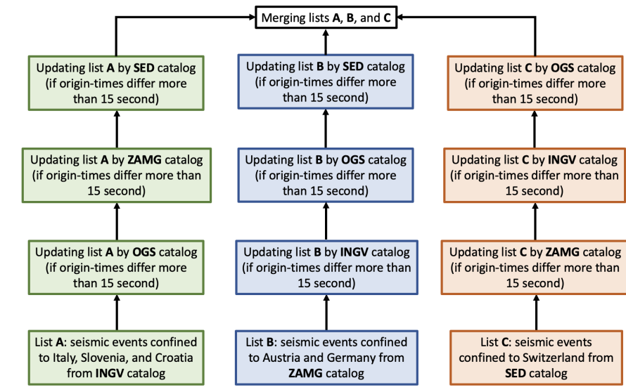
Figure A1. Flow chart showing the process of merging seismic catalogs of INGV, OGS, ZAMG, and SED in order to derive an integrated seismic event list in the study region.
