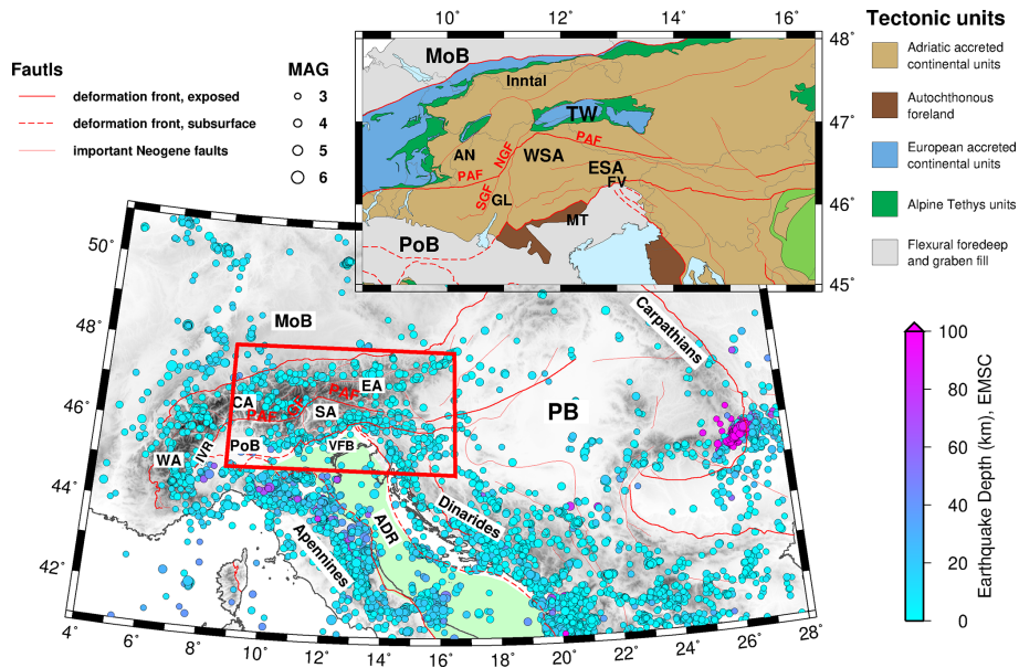
Figure 1. Geological map of the Alps showing major deformation fronts, faults, geographical subdivisions, tectonic units, and seismicity (seismic events between January 2000 and December 2012 with a magnitude larger than 3 from the European-Mediterranean Seismological Centre). The light green zone indicates the outline of the Adriatic plate. The tectonic units of the study area (red box) are shown on the upper-right inset map. The maps are modified from Handy et al. (2010) and Schmid et al. (2004, 2008). Abbreviations are as follows: WA stands for western Alps, CA stands for central Alps, SA stands for southern Alps, EA stands for eastern Alps, ADR stands for Adriatic plate, IVR stands for Ivrea body, PB stands for Pannonian Basin, VFB stands for Venetian-Friuli Basin, PoB stands for Po Basin, MoB stands for Molasse Basin, TW stands for Tauern Window, PAF stands for Periadriatic Fault, NGF stands for northern Giudicarie Fault, SGF stands for southern Giudicarie Fault, ESA stands for eastern southern Alps, WSA stands for western southern Alps, MT stands for Montello, GL stands for Giudicarie–Lessini region, FV stands for Friuli-Venetia region, and AN stands for Austroalpine nappes.
