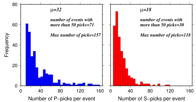
Figure 4. Histograms of high-quality P and S picks per event for 301 well-constrained local earthquakes used for simultaneous inversion of hypocenters, 1-D velocity models, and station corrections.
