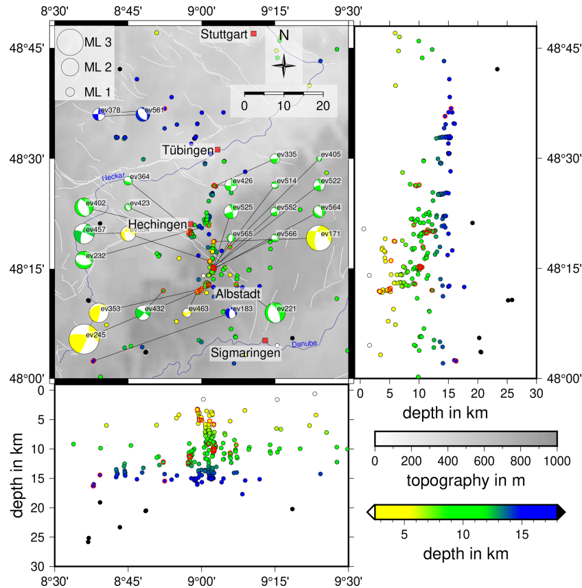
Figure 7. Hypocenters of the 337 best-located events with a horizontal error of less than 1 km and a depth error of less than 2 km. Only events with a GAP smaller than 180^\circ and more than eight travel time picks are included. Hypocenters are plotted as circles that are color-coded by depth. All 25 focal mechanisms are displayed also color-coded by depth; red circles indicate the corresponding event hypocenter. The size of the focal mechanisms is scaled depending on ML of the event. Cluster codes are placed next to the fault plane solutions. White lines indicate known and assumed faults (Regierungspräsidium Freiburg, 2019). Topography is based on the ETOPO1 Global Relief Model (Amante and Eakins, 2009; NOAA National Geophysical Data Center, 2009).
