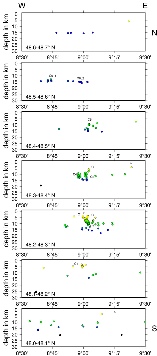
Figure 10. Seismicity distribution of the ASZ from north (top) to south (bottom). Circles indicate hypocenters in the corresponding slice, color-coded by depth (as in Fig. 7); cluster codes are given for orientation.
