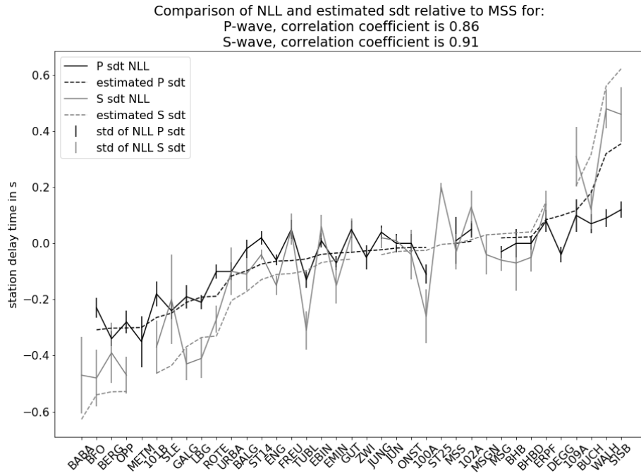
Figure 9. Comparison of NLL station delay times (sdt) and estimated station delay times due to depth variations of the crystalline basement: P waves (black) and S waves (gray). Stations along the x axis are sorted from shallow to deep crystalline basement model depth.
