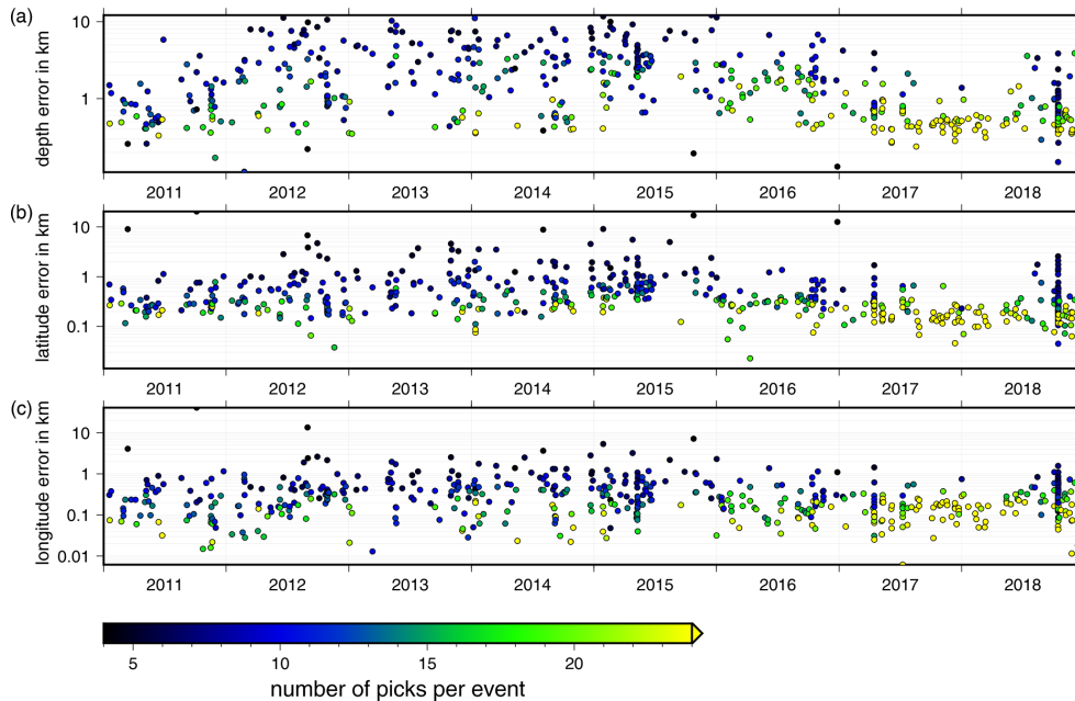
Figure 5. Errors calculated from the 68 % confidence ellipsoid from NLL with L2 (L2-rms likelihood function) for each event in the combined catalog for (a) depth, (b) latitude and (c) longitude. The errors are color-coded depending on the number of picks, with dark colors indicating fewer picks and bright colors indicating many picks. Hypocenters with many observations are determined with smaller errors in depth and lateral position.
