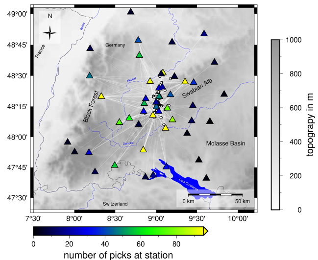
Figure 2. Ray coverage and input data set for the inversion with VELEST. White circles represent the 99 selected events that are used for v_p and v_s inversion. Seismic stations are indicated as triangles and color-coded with the number of high-quality picks at a station used for the v_p and v_s inversion. Topography is based on the ETOPO1 Global Relief Model (Amante and Eakins, 2009; NOAA National Geophysical Data Center, 2009).
