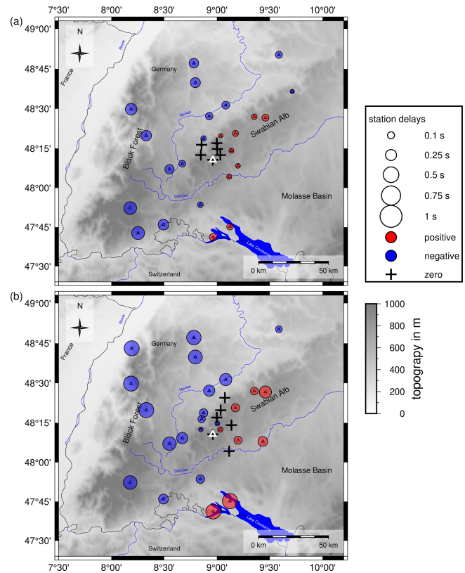
Figure 6. (a) Station delay times for the v_p velocity model ASZmod1. (b) Station delay times for the v_s velocity model ASZmod1. Blue circles represent negative station delay times, indicating areas with faster velocities than ASZmod1. Red circles illustrate positive station delay times, indicating slower velocities than ASZmod1. Crosses are stations with zero station delays. Only stations with more than five travel time picks are included. The small white triangle highlights reference station MSS. Topography is based on the ETOPO1 Global Relief Model (Amante and Eakins, 2009; NOAA National Geophysical Data Center, 2009).
