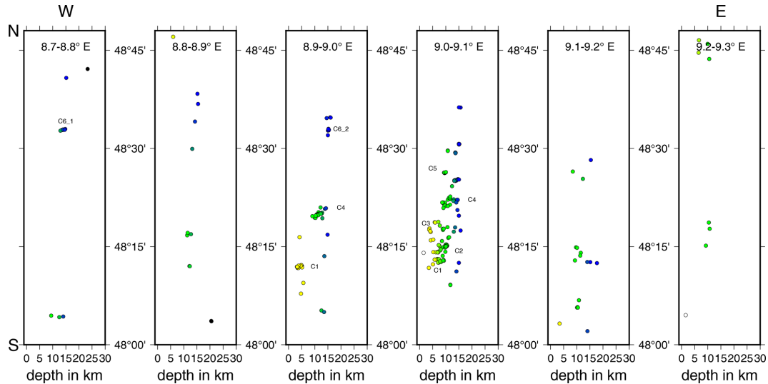
Figure 11. Seismicity distribution of the ASZ from west (left) to east (right). Circles indicate hypocenters in the corresponding slice, color-coded by depth (as in Fig. 7); cluster codes are given for orientation.
