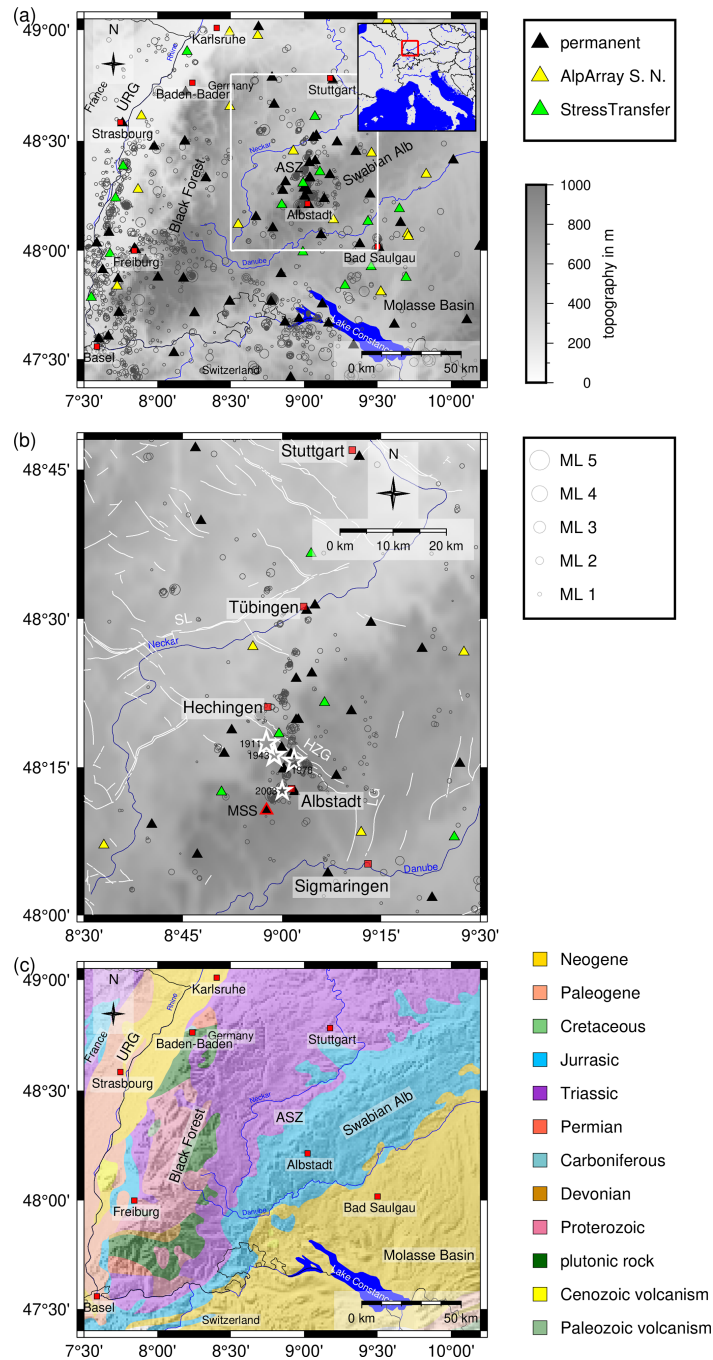
Figure 1. (a) Overview over our research area located in southwestern Germany in the northern Alpine foreland. The ASZ is our research target (framed area). Black triangles represent permanent seismic stations of the LED and other agencies. Yellow triangles represent temporary AlpArray seismic stations. Green triangles display the 15 temporary seismic stations of the StressTransfer network. The gray circles display the seismicity scaled by magnitude from 2011 to 2018. URG stands for Upper Rhine Graben. (b) Close-up of the area of the ASZ (framed area in (a)). Symbols are the same as in (a). The red-framed triangle highlights the central station Meßstetten (MSS) of the minimum 1-D seismic velocity model. White stars mark epicenters of the four strongest events, which had a magnitude greater than 5 in 1911, 2 in 1943 (same epicenter) and 1978, as well as the earthquake on 22 March 2003 with a local magnitude of 4.4 (Leydecker, 2011) these events are not included in the earthquake catalog from 2011 to 2018 (gray circles scaled with magnitude like in Fig. 1a). White lines indicate known and assumed faults (Regierungspräsidium Freiburg, 2019). The Hohenzollern Graben (HZG) is the only clear morphological feature in the close vicinity of the ASZ. Other large tectonic features are the Lauchert Graben (LG) and the Swabian Line (SL). Topography is based on the ETOPO1 Global Relief Model (Amante and Eakins, 2009; NOAA National Geophysical Data Center, 2009). (c) Overview on the geology of the research area region; geology data are taken from Asch (2005). Topography is based on SRTM15+ (Tozer et al., 2019).
