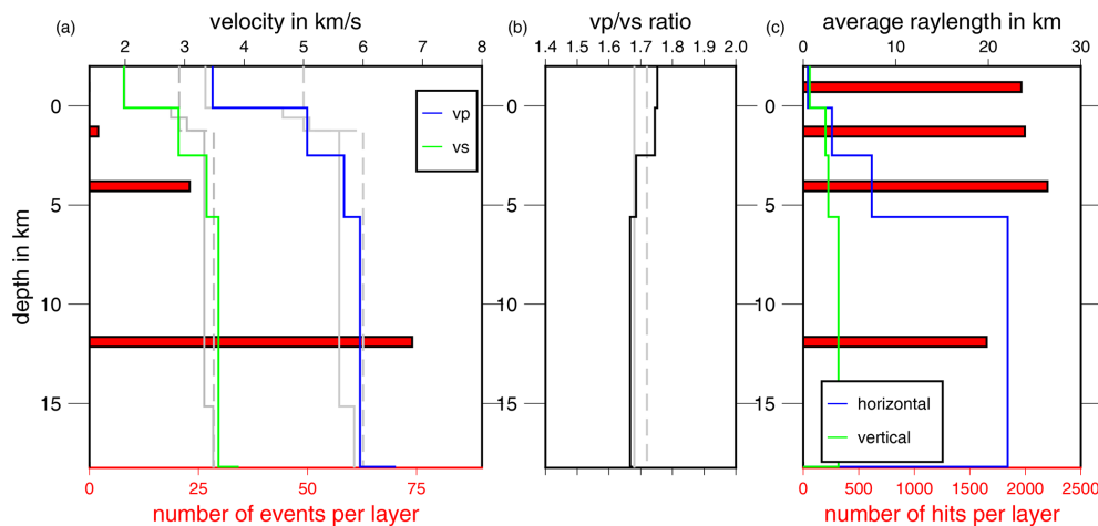
Figure 4. (a) Final minimum 1-D seismic velocity models (ASZmod1): v_s is in green, and v_p is in blue. Gray lines represent velocity models of the LED (Bulletin-Files des Landeserdbebendienstes B-W, 2018): solid lines show Swabian Jura models, and dashed lines show Baden-Württemberg models. Red bars are scaled with the number of events in each layer of the velocity model. (b) v_p/v_s ratio of ASZmod1 and the LED models. (c) Ray statistics of used ray paths. Red bars display number of hits per layer. Blue and green lines give the average horizontal and vertical ray length.
