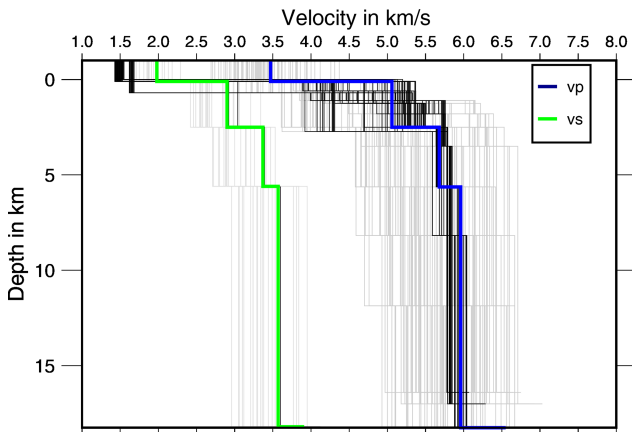
Figure 3. VELEST input models for v_p (84) and v_s (21) (gray) and output v_p (84) and v_s (21) after inversion (black) together with the chosen model ASZmod1 (colored). A good convergence of the models can be observed, especially for v_s . The second layer converges worst. An instability of the first layer with a tendency to unrealistic low seismic velocities can be seen. For this reason, the velocity of ASZmod1 was fixed in the first layer.
