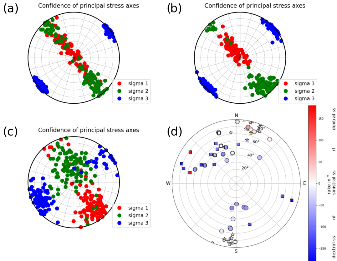
Figure 8. (a) Confidence plot of the principal stress axes \sigma_1 , \sigma_2 and \sigma_3 after the stress inversion of all fault plane solutions (Table 2) for the 100 different noise realizations. (b) The same as Fig. 8a but only for fault plane solutions with a depth greater than 7.5 km. (c) The same as Fig. 8a but only for fault plane solutions with a depth less than 7.5 km. (d) Strike, dip and rake of all measured fault plane solutions (circles). The yellow star represents strike and dip of the 22 March 2003 earthquake (Stange and Brüstle, 2005). Other stars represent fault plane solutions calculated by Turnovsky (1981) for the earthquake series in 1978. Fault planes of StressInverse (Vavryčuk, 2014) are displayed by squares. Negative rake angles hint at normal faulting (nf) components, and positive angles hint at reverse faulting (rf) components. Events with a rake close to zero exhibit sinistral strike-slip (sinistral ss) components; events with rake angles close to -180 or 180^\circ hint to dextral strike-slip (dextral ss).
