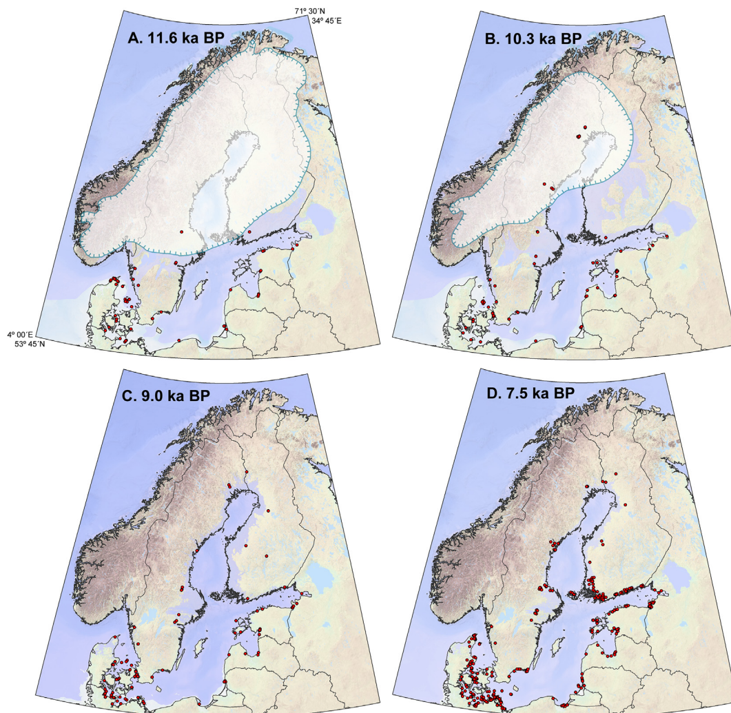
Fig. 2. Holocene development of the BSB with accepted RSL data points (red dots) from the (A) Yoldia Sea; (B) Ancylus Lake; (C) Initial Littorina Sea, and (D) Littorina Sea stages. The extent of the water bodies in BSB (semitransparent blue areas) is compiled according to data by Andrén et al. (2011) , Eronen et al. (2001) and Rosentau et al. (2012) . Topographic data from EMODnet Bathymetry. (For interpretation of the references to colour in this figure legend, the reader is referred to the Web version of this article.)
