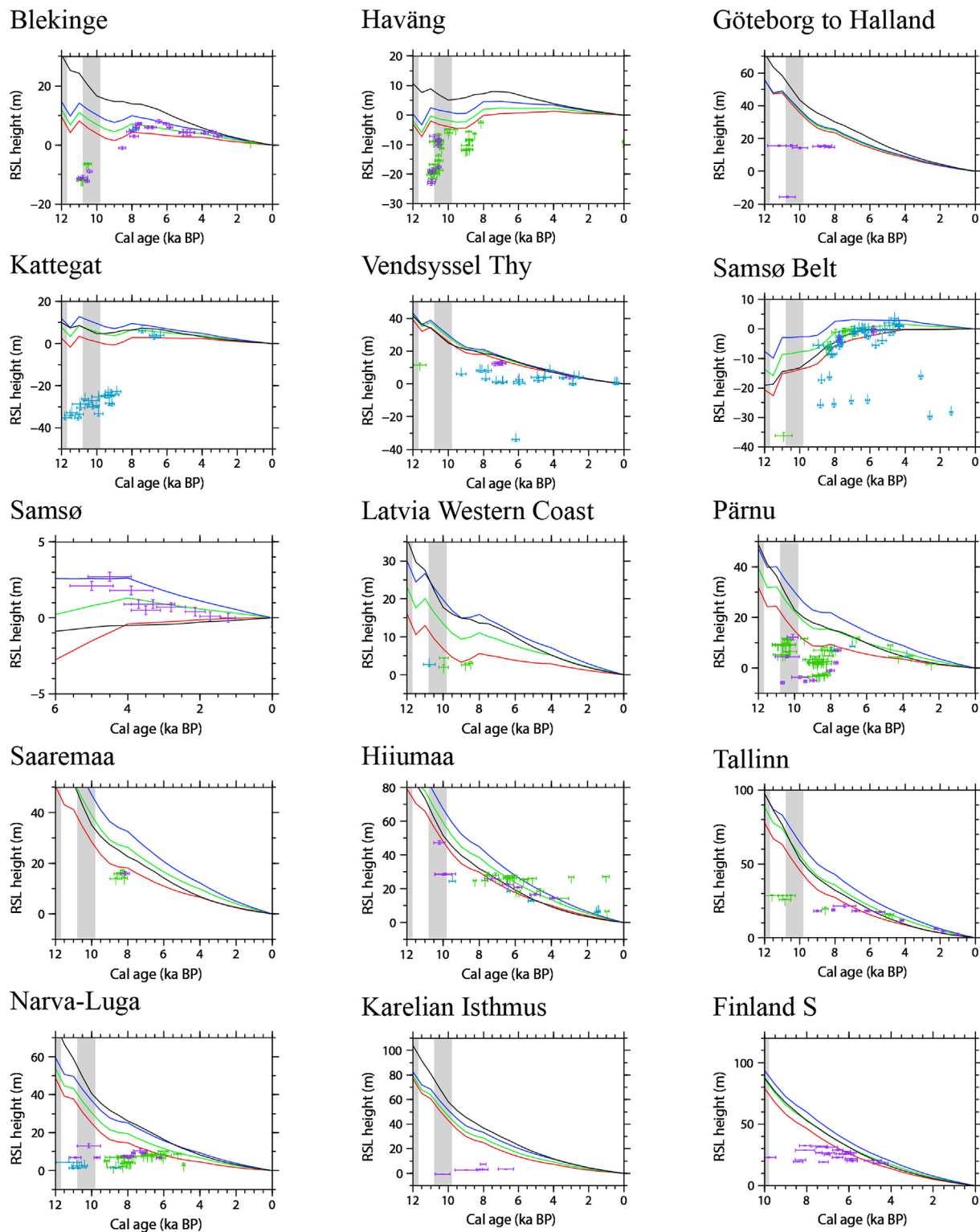
Fig. 8. RSL data showing the complex tendencies and predictions considering ICE-5G with three different lithosphere thicknesses and ICE-6G_C(VM5a). For details see Fig. 7.
