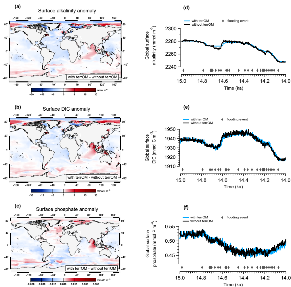
Figure 8. Anomaly of the mean surface alkalinity (a), surface dissolved inorganic carbon (b), and surface phosphate (c) between the two simulations with and without terrestrial organic matter fluxes averaged over MWP1a. Time evolution of the two simulations during MWP1a for annual mean global surface alkalinity (d), DIC (e) and phosphate (f).
