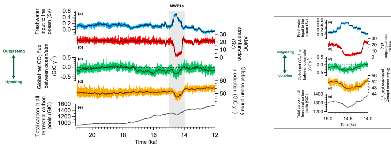
Figure 2. Land-ocean-atmosphere comparison during the last deglaciation. The presented outputs start at 21 ka, after the spin-up runs between 26-21 ka. (a) Freshwater input to the global ocean. (b) Atlantic Meridional Overturning Circulation streamfunction. (c) Global net \text{CO}_2 flux between the ocean and the atmosphere. Positive values mean that the ocean is outgassing to the atmosphere and negative values that the ocean is uptaking carbon. (d) Global ocean primary production. (e) Total carbon in all terrestrial carbon pools, i.e. vegetation, soil and litter. The thick darker curves are 500 years running mean for the freshwater input and 50 years running mean for the other panels. A zoom over Meltwater Pulse 1a is presented on the right.
