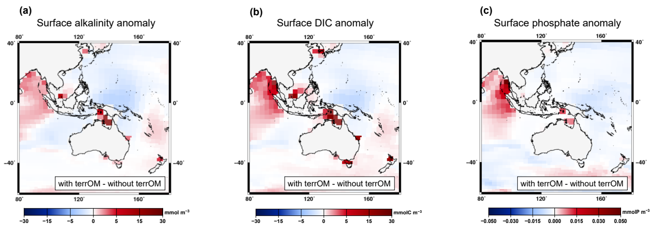
Figure 9. Same as Fig. 8a, b, c but with a focus over Indonesia for the surface alkalinity (a), surface dissolved inorganic carbon (b) and surface phosphate (c) between the two simulations with and without terrestrial organic matter fluxes averaged over MWP1a.
