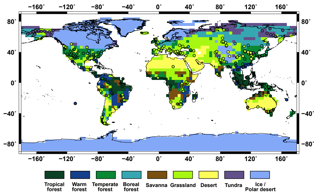
Figure 4. Biome distribution modelled by JSBACH at 15 ka. The superimposed circles are the pollen data from the BIOME6000 Version 4.2 reconstruction at 21 ka (Harrison, 2017).
