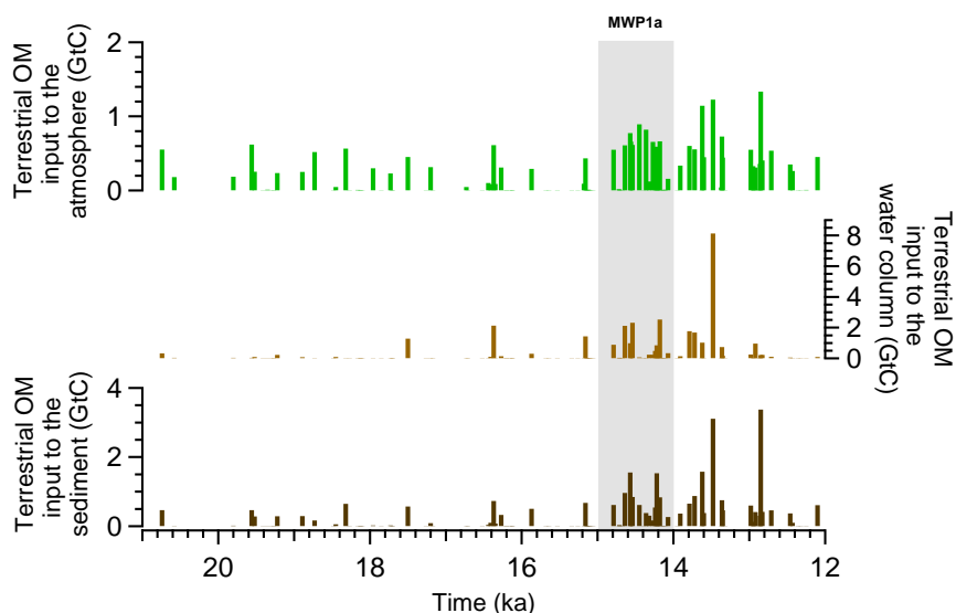
Figure 6. Time series of terrestrial organic matter inputs during the last deglaciation. Top panel: Terrestrial organic matter (vegetation, green biomass and non-woody litter) inputs to the atmosphere. Middle panel: Terrestrial organic matter (wood and woody litter above ground) inputs to the water column and to the water-sediment interface. Bottom panel: Terrestrial organic matter (woody litter below ground and humus) inputs to the sediment.
