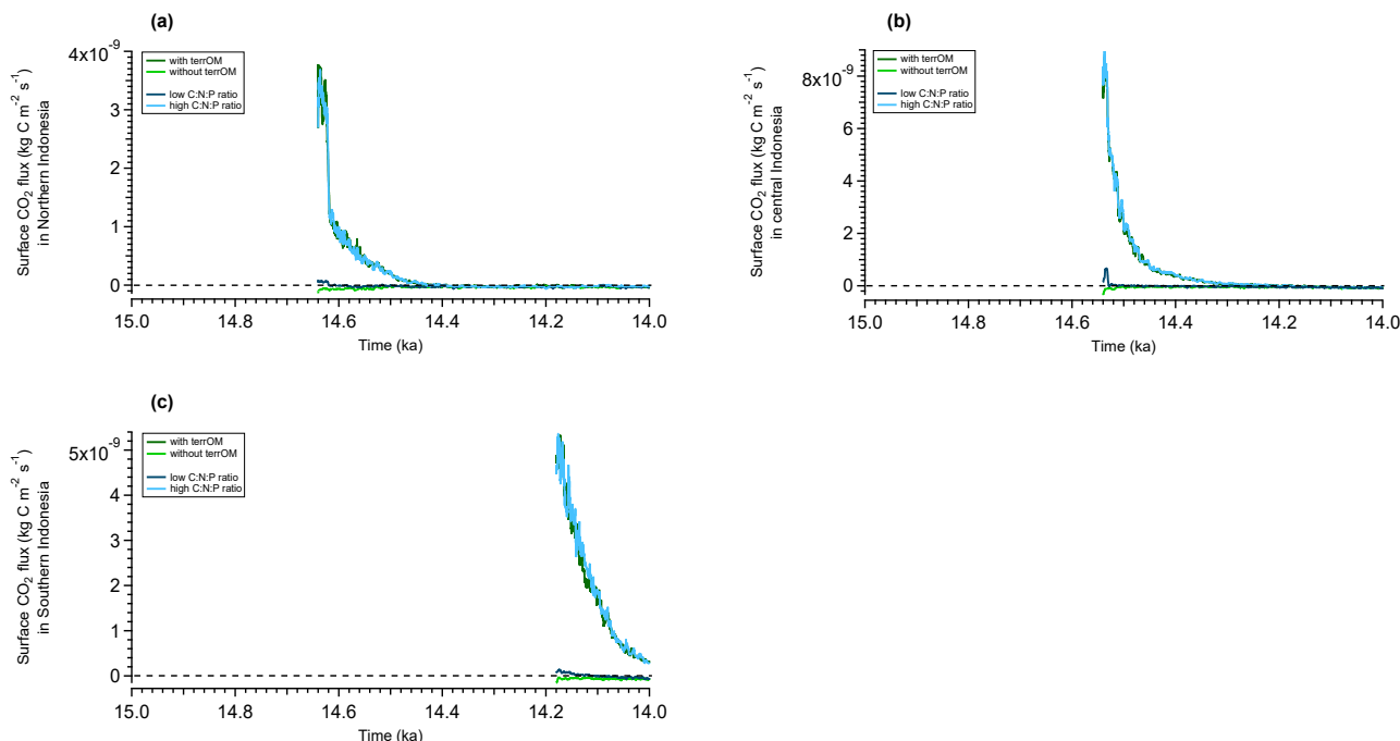
Figure 11. Evolution of the surface CO 2 flux during MWP1a for flooded grid cells in Northern (a), central (b) and Southern Indonesia (c) for 4 simulations: the reference simulation with the terrestrial organic matter fluxes (dark green), the sensitivity experiment without terrestrial organic matter fluxes (light green), the sensitivity experiment with low stoichiometry for terrestrial organic matter (dark blue) and the sensitivity experiment with high stoichiometry (light blue). 50 years running mean are plotted for each simulation. Positive values indicate an outgassing to the atmosphere and negative values indicate an uptake by the ocean.
