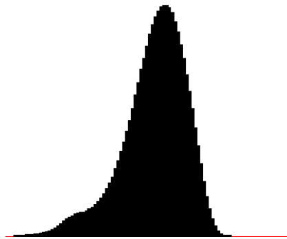
Figure 3: Dihedral angles histogram from 0 to 90°.
