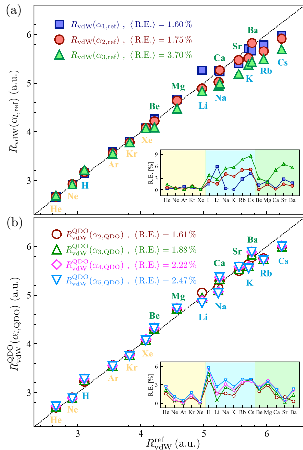
FIG. 3. The vdW radius as a function of the multipole polarizabilities, R_{\text{vdW}}(\alpha_l) = A_l \alpha_l^{2/7(l+1)} , obtained by means of (a) Eqs. (42) and (b) Eqs. (43), is presented, taking into account that R_{\text{vdW}}^{\text{QDO}}(\alpha_{l,\text{QDO}}) \equiv R_{\text{vdW}}(\alpha_{l,\text{ref}}) , in comparison to the reference values R_{\text{vdW}}^{\text{ref}} [24,85,86] for three classes of species: Noble gases (in yellow), H + alkali-metal atoms (group I, in blue), and alkaline-earth atoms (group II, in green). The vdW radii are shown (a) for the reference [33,77–79] multipole polarizabilities \alpha_{1,\text{ref}} , \alpha_{2,\text{ref}} , and \alpha_{3,\text{ref}} (blue, red, and green filled symbols) and (b) for the QDO multipole polarizabilities \alpha_{2,\text{QDO}} , \alpha_{3,\text{QDO}} , \alpha_{4,\text{QDO}} , and \alpha_{5,\text{QDO}} given by Eq. (6) (red, green, fuchsia, and light blue open symbols). The insets show the relative errors, \text{R.E.} = |R_{\text{vdW}}(\alpha_l) - R_{\text{vdW}}^{\text{ref}}|/R_{\text{vdW}}^{\text{ref}} , for the noble gases (yellow box), the alkali metals + hydrogen (light blue box), and the alkaline-earth elements (light green box). In addition, the mean values of the relative errors, (R.E.), are reported in the legends, for each considered multipole order.
