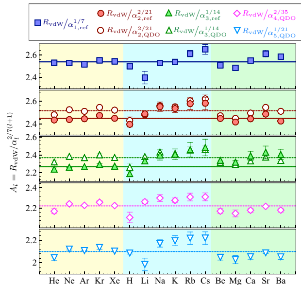
FIG. 2. The ratios R_{\text{vdW}} / \alpha_{l,\text{ref}}^{2/7(l+1)} listed in Table I are shown (filled symbols) with respect to the “universal” values A_1 = 2.54 a.u., A_2 = 2.45 a.u., and A_3 = 2.27 a.u., represented with blue, red, and green solid lines, respectively. By contrast, the ratios R_{\text{vdW}} / \alpha_{l,\text{QDO}}^{2/7(l+1)} (open symbols) are plotted with respect to the constant values obtained from the QDO polarizabilities, A_2^{\text{QDO}} = 2.52 a.u., A_3^{\text{QDO}} = 2.37 a.u., A_4^{\text{QDO}} = 2.23 a.u., and A_5^{\text{QDO}} = 2.10 a.u., shown with red, green, fuchsia, and light blue dotted lines, respectively. The noble gases are shown in the yellow box, the elements of group I are shown in the light blue box, and the elements of group II are shown in the light green box. The error bars represent the relative errors \text{R.E.} = |A_l[X] - A_l| / A_l of each species X , where A_l are the universal values expressed in Eqs. (42) for the ratios R_{\text{vdW}} / \alpha_{l,\text{ref}}^{2/7(l+1)} and in Eqs. (43) for R_{\text{vdW}} / \alpha_{l,\text{QDO}}^{2/7(l+1)} .
