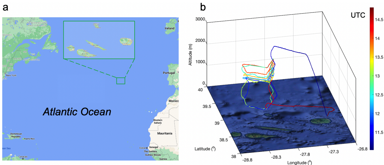
Figure 2. (a) The geographical location of the ACE-ENA campaign. (b) An example of a representative flight pattern on 25 January 2018. The G-1 flew an L-shaped pattern consisting of along-wind legs upwind of Graciosa Island and cross-wind legs over the ocean. Maps are obtained from © Google Maps.
