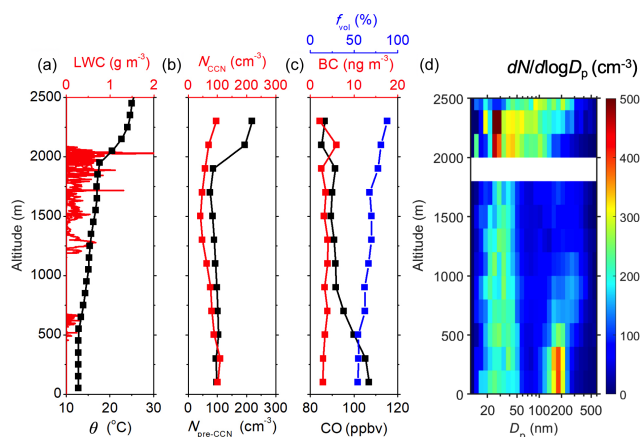
Figure 10. Vertical profiles of parameters under the synoptic condition of pre-front on 8 February 2018. (a) Potential temperature ( \theta ) and liquid water content (LWC). (b) N_{\text{pre-CCN}} and N_{\text{CCN}} . (c) Concentrations of carbon monoxide (CO) and black carbon (BC), as well as the aerosol volatile fraction ( f_v ). (d) Vertical contour of aerosol size distributions as a function of altitude. Size distributions between 1800 and 2000 m are not shown due to the interference of cloud droplet shattering. The CO mixing ratio, BC concentration, particle concentrations, and size distributions are normalized to standard temperature and pressure (273.15 K and 101.325 kPa; STP).
