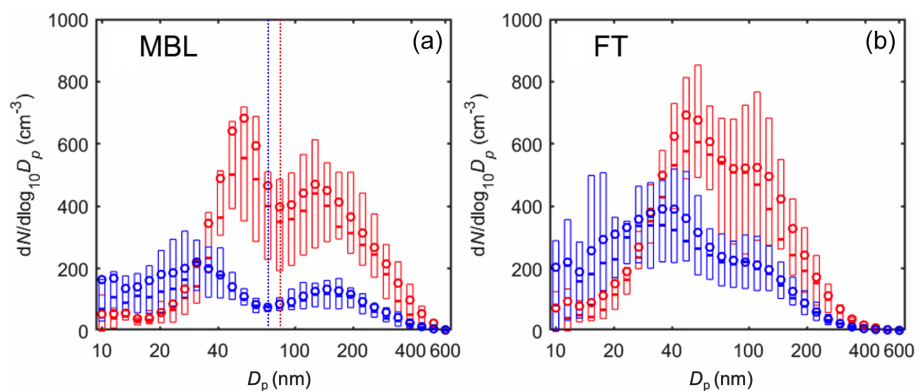
Figure 5. Aerosol size distributions measured by the FIMS on board the G-1 aircraft within (a) the MBL and (b) lower FT during the summer IOP (red) and winter IOP (blue). The line and circle markers represent the median and mean of the size distribution, and the edges of the box indicate the 25th and 75th percentiles, respectively. The dotted lines in panel (a) show the Hoppel minimum for the averaged size distributions in the MBL.
