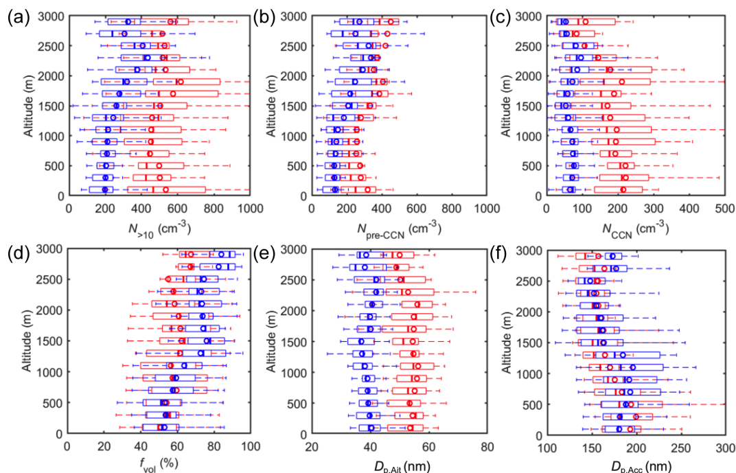
Figure 6. Vertical profiles showing the (a) concentration of particles larger than 10 nm ( N_{>10} ), (b) concentration of Aitken-mode aerosols or aerosols too small to form cloud droplets ( N_{\text{pre-CCN}} ), (c) concentration of accumulation-mode aerosols or CCN ( N_{\text{CCN}} ), (d) aerosol volatile fraction ( f_{\text{vol}} ), (e) average size of Aitken-mode aerosol ( D_{p,\text{Ait}} ), and (f) average size of accumulation-mode aerosol ( D_{p,\text{Acc}} ) over the ENA site during the summer IOP (red) and winter IOP (blue). The concentrations are normalized to standard temperature and pressure (273.15 K and 101.325 kPa; STP). The line and circle markers represent the median and mean of the data, and the edges of the box indicate the 25th and 75th percentiles, respectively.
