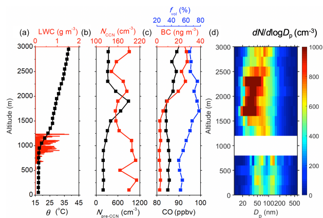
Figure 9. Vertical profiles of parameters under the synoptic condition of Azores high on 8 July 2017. (a) Potential temperature ( \theta ) and liquid water content (LWC). (b) N_{\text{pre-CCN}} and N_{\text{CCN}} . (c) Concentrations of carbon monoxide (CO) and black carbon (BC), as well as the aerosol volatile fraction ( f_{\text{vol}} ). (d) Vertical contour of aerosol size distributions as a function of altitude. Size distributions between 800 and 1200 m are not shown due to the interference of cloud droplet shattering. The CO mixing ratio, BC concentration, particle concentrations, and size distributions are normalized to standard temperature and pressure (273.15 K and 101.325 kPa; STP).
