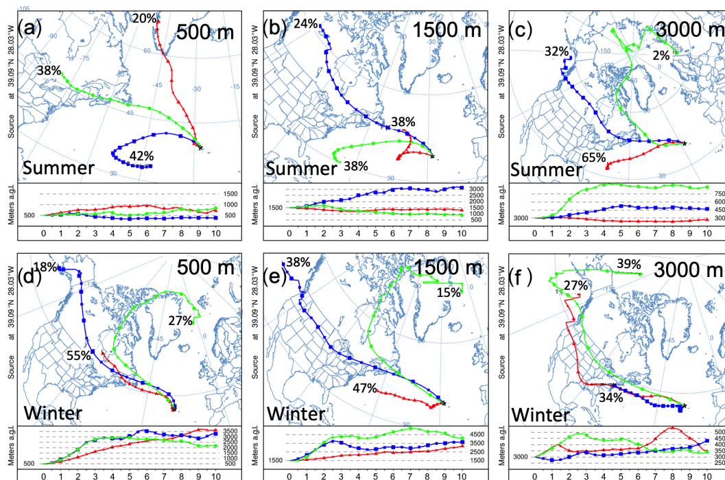
Figure 3. Cluster analysis of 10 d back trajectories arriving at 500, 1500, and 3000 m above the ENA site during the summer (a)–(c) and winter (d)–(f) IOP. The average 10 d back trajectories of the three clusters are represented by red, green, and blue lines, and the associated numbers denote the occurrence percentages of the clusters.
