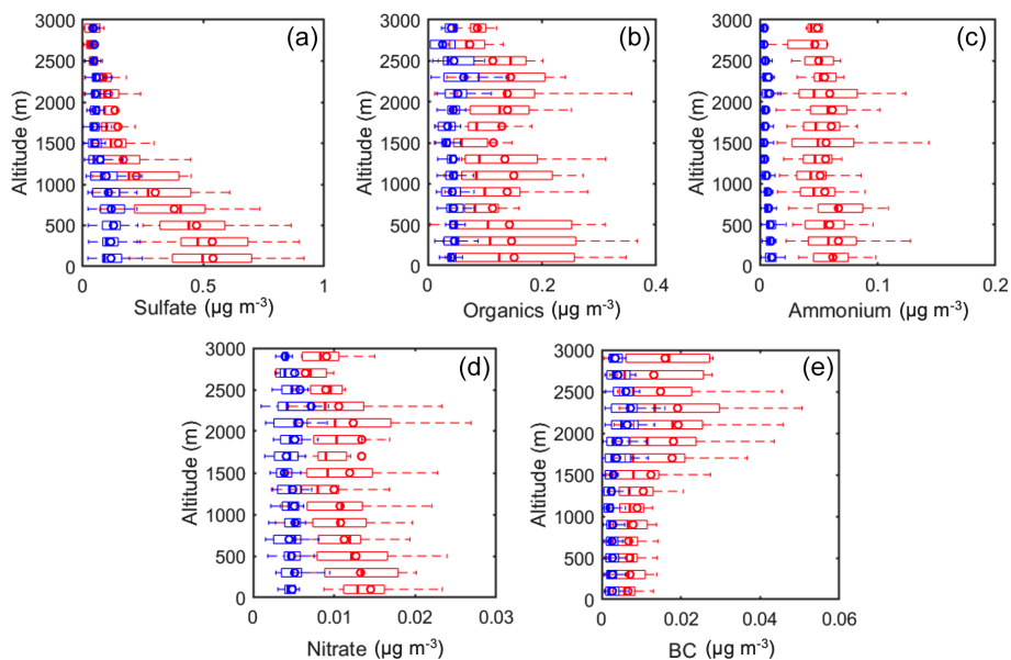
Figure 7. Vertical profiles of the mass concentrations of (a) sulfate, (b) organics, (c) ammonium, (d) nitrate, and (e) black carbon (BC) in the ENA during the summer IOP (red) and winter IOP (blue). BC is measured by the SP2, and the rest of the compositions are measured by the HR-ToF-AMS. The line and circle markers represent the median and mean of the data, and the edges of the box indicate the 25th and 75th percentiles, respectively. The concentrations are normalized to standard temperature and pressure (273.15 K and 101.325 kPa; STP).
