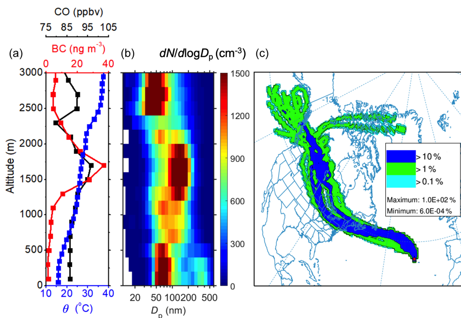
Figure 8. A long-range transport event observed during the research flight on 29 June 2017. (a) Vertical profiles of potential temperature ( \theta ), black carbon (BC) mass concentration, and carbon monoxide (CO) mixing ratio. (b) Vertical contour of aerosol size distributions as a function of altitude measured by the FIMS. (c) Frequency analysis of hourly back trajectories arriving at the ENA site on 29 June 2017 generated by HYSPLIT. The frequency is the sum of the number of trajectories that passed through each grid cell divided by the total number of trajectories analyzed. The CO mixing ratio, BC concentration, and size distributions are normalized to standard temperature and pressure (273.15 K and 101.325 kPa; STP).
