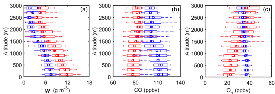
Figure 4. Vertical profiles of (a) water vapor mixing ratio ( w ), (b) carbon monoxide mixing ratio (CO), and (c) ozone mixing ratio ( O_3 ) over the ENA site during the summer IOP (red) and winter IOP (blue). The mixing ratios are normalized to standard temperature and pressure (273.15 K and 101.325 kPa; STP). The line and circle markers represent the median and mean concentrations, and the edges of the box indicate the 25th and 75th percentiles, respectively.
