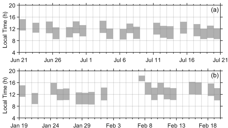
Figure 1. Date and time periods of research flights during summer (a) and winter (b) IOPs of the ACE-ENA campaign.
