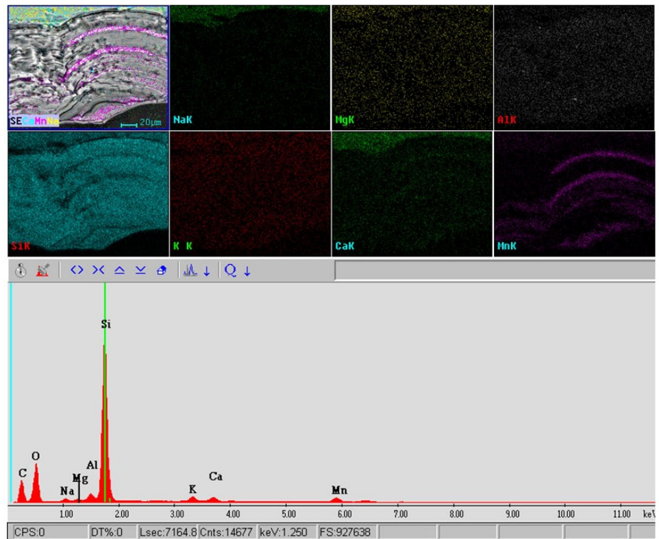
Figure 8. SEM-EDS elemental mapping of the chemical composition (glass fragment KK_d12, cross-section). Scale bar is the same for all subfigures.
