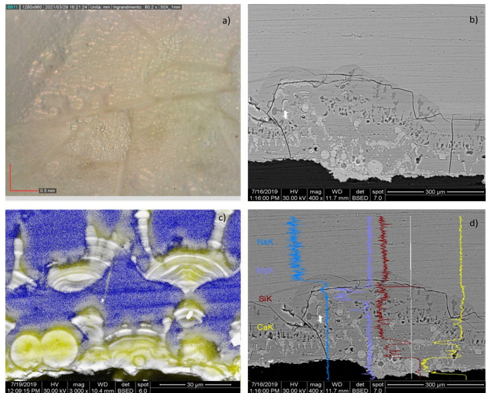
Figure 5. Sample KK_d11: (a) OM documentation; (b) BSE image of the cross-section, with detail of the alteration layer; (c) SEM-EDS mapping, with details of Ca (yellow) and Si (blue) contents; (d) EDS line scan through the altered surface and the pristine glass.
