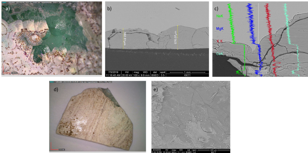
Figure 4. Opaque weathering: (a) OM documentation of fragment KK_b2; (b) BSE image of KK_b2 cross-section, with detail of the alteration layer penetrating inside the glass; (c) EDS line scan through the altered surface and the pristine glass; (d) OM documentation of fragment KK_d7, with enamel-like weathering; (e) BSE images of fragment KK_d7, untreated sample.
