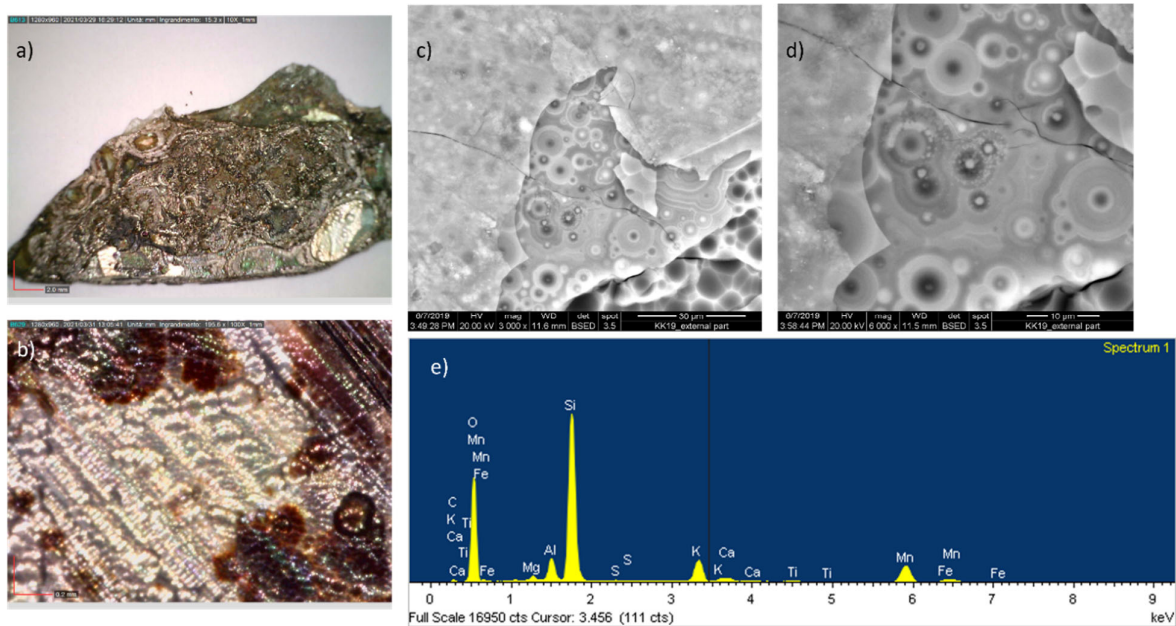
Figure 7. Blackening alteration: (a) OM documentation of fragment KK_d12; (b) detail of black stains under OM (100×); (c,d) BSE images of the lamellar structure, with details of concentric pits; (e) EDS spectrum acquired on the pits.
