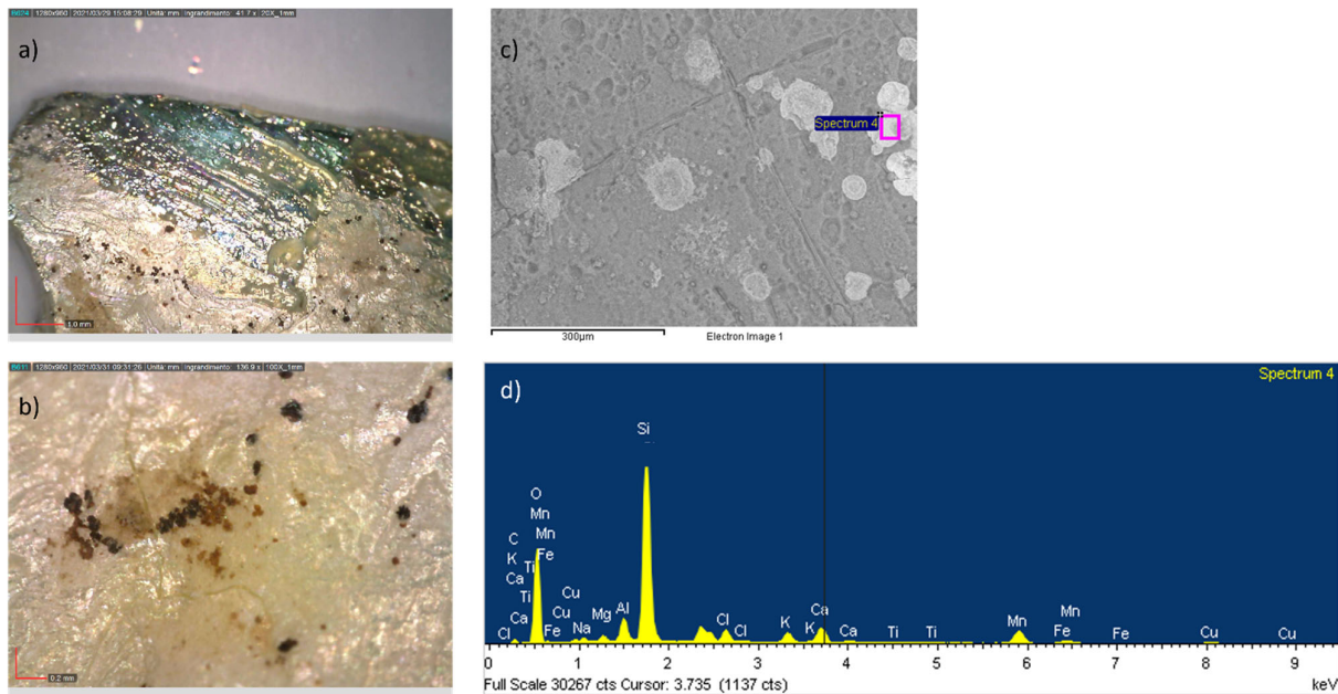
Figure 3. Iridescence on glass fragment KK_d3: (a) OM documentation; (b) magnified detail of the black stains (100×); (c) BSE image of the surface; (d) EDS spectrum acquired on the black stains.
