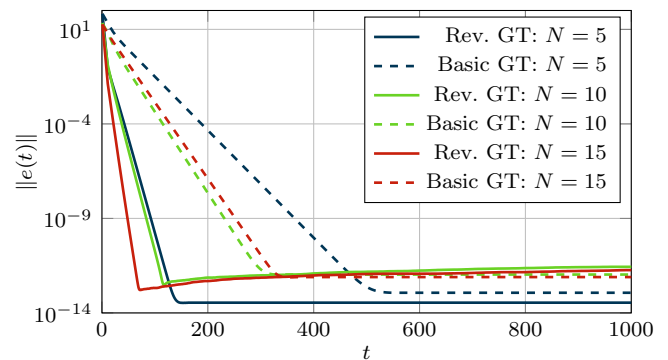
Fig. 1. Evolution of error e(t) for different values of N .
