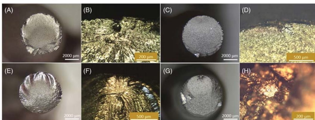
FIGURE 4 Fracture surfaces observed by stereoscope (A, C, E, G) and by optical microscope (B, D, F, H). Sample numbers: NN08 (A, B); HN05 (C, D); NM05 (E, F); HM13 (G, H) [Colour figure can be viewed at wileyonlinelibrary.com ]
