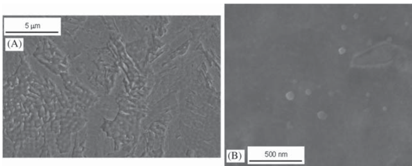
FIGURE 9 Scanning electron microscope (SEM-FEG) observations in the not heat treated state: (A) equiaxed and columnar cell structures and (B) observed precipitates
