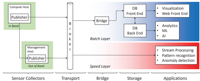
Fig. 1: ExaMon Architecture
