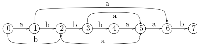
Figure2. Factor oracle of \text{abbbaab} . The word aba is recognizes whereas it is not a factor.
