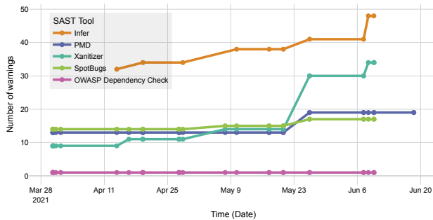
Figure 3: Security-related warnings in our SAST database queried for the luca App for Android ( https://gitlab.com/lucaapp/android ).
