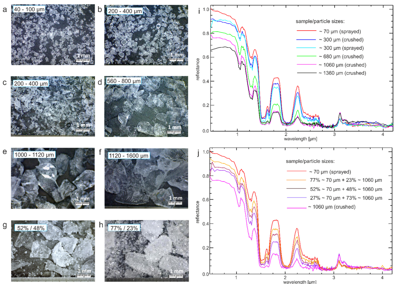
Figure 1. Left column: optical images of the samples prepared for the study with particle sizes of (a) ~70 \mu m, (b): sprayed ~300 \mu m; (c): crushed ~300 \mu m, (d) ~680 \mu m, (e) ~1060 \mu m, (f) ~1360 \mu m and examples of particle size mixtures such as (g) 52%~70 \mu m + 48%~1060 \mu m, and (h) and 77%~70 \mu m + 23%~1060 \mu m. Right column: resulting spectra of the samples at different particle sizes (i) and of the particle size mixtures (j) over the entire wavelength interval (0.4–4.2 \mu m) measured at 70 K.
