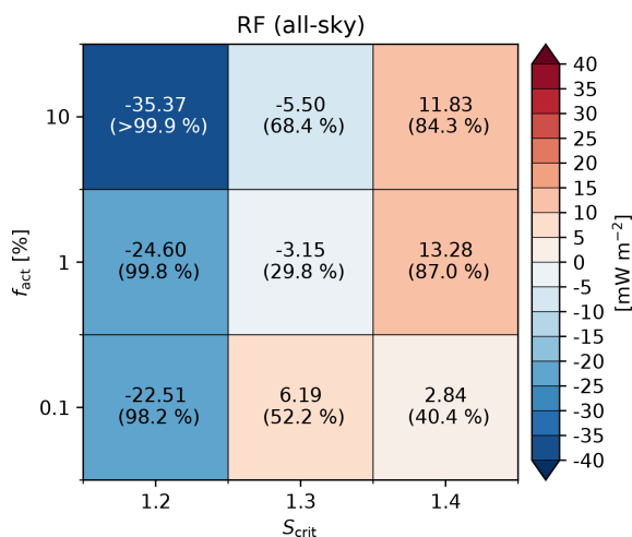
Figure 5. Multi-year average (2001–2015) top-of-the-atmosphere all-sky RF due to the effect of aviation soot on natural cirrus clouds, under different assumptions for the ice nucleation efficiency of aviation soot INPs ( S_{\text{crit}} and f_{\text{act}} ). The values in brackets within each box indicate the confidence level.
