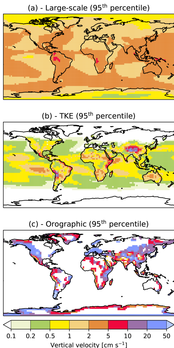
Figure 2. The vertical velocity components considered by the model: (a) large-scale, (b) subscale using the turbulent kinetic energy (TKE) as proxy, and (c) subscale contribution of the orographic waves in the vicinity of mountain ranges. Each panel shows the 95th percentile of the vertical velocity distribution with respect to the time (over the 2001–2015 simulation period) and vertical (above 400 hPa) coordinates.
