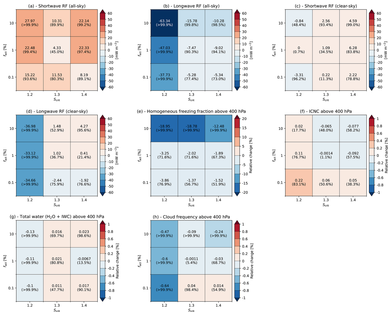
Figure 6. As in Fig. 5 but for (a) all-sky shortwave, (b) all-sky longwave, (c) clear-sky shortwave, and (d) clear-sky longwave top-of-the-atmosphere RFs. Panels (e–h) depict the aviation-soot-induced relative changes in ICNC from homogeneous freezing, ICNC, total water (as the sum of water vapour and ice water), and cloud frequency, respectively, all spatially averaged above 400 hPa and over cloudy and cloud-free model grid boxes.
