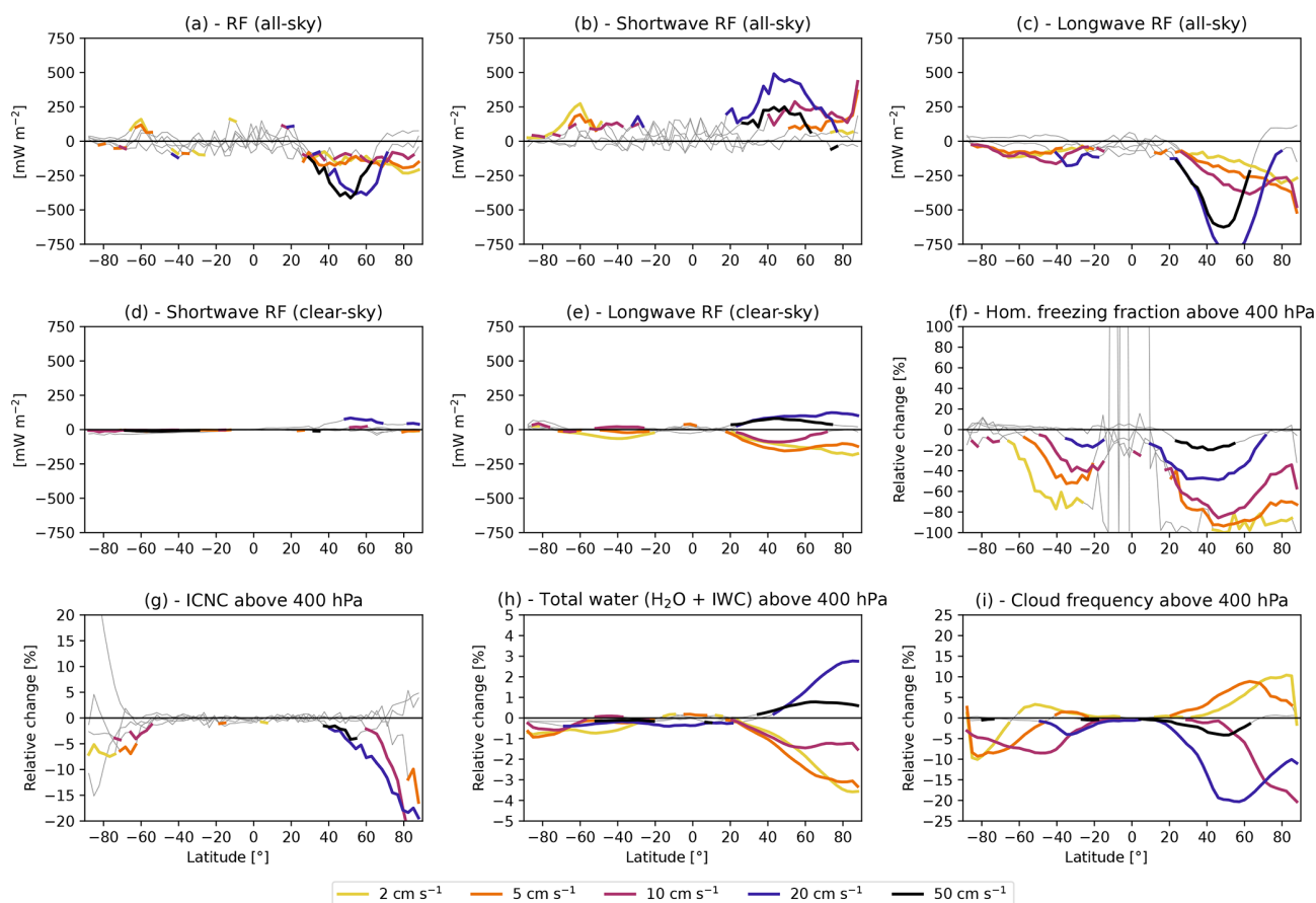
Figure 9. As Fig. 8 but showing zonal averages. Values with a statistical significance below 95 % are drawn in grey.
