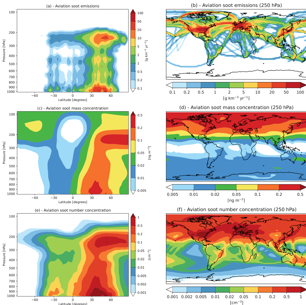
Figure 4. Aviation soot emissions from the CMIP6 dataset used for the model simulations in this work (a, b). The other panels show the mass concentration (c, d) and the number concentration (e, f) of aviation soot simulated by EMAC-MADE3 (BASE experiment; see Table 1). Panels (a), (c), and (e) show zonal means, whereas (b), (d), and (f) show the \sim 250 hPa level. All panels consider the multi-year average over the simulated period (2001–2015). Note that the number concentration of aviation soot is further multiplied by the active fraction f_{\text{act}} = 0.1\%–10\% in the cirrus parametrization to obtain the number concentration of aviation soot INPs.
